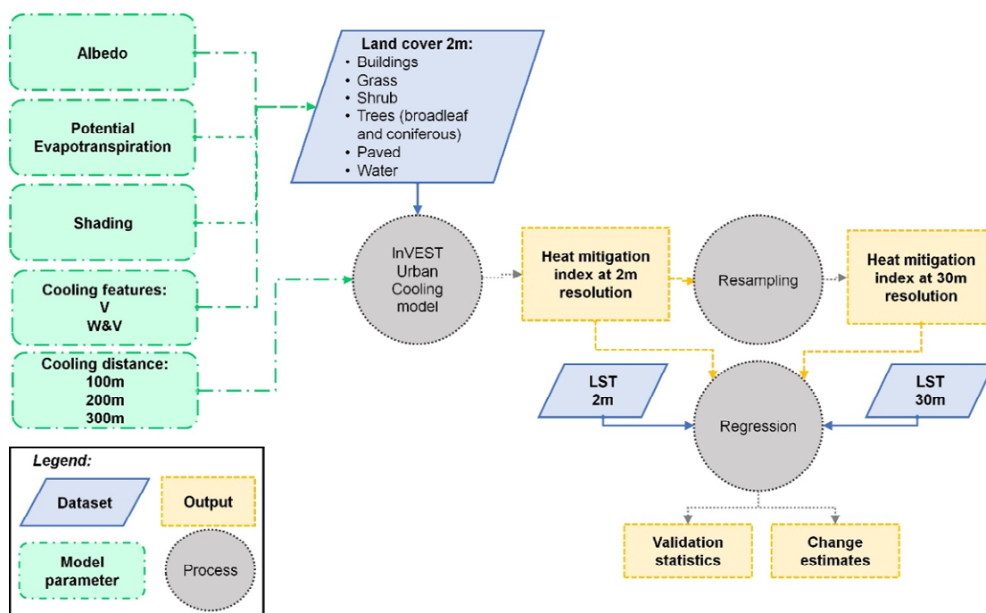
Figure 2 Schematic of the methodology undertaken to assess the representativeness of the heat mitigation index derived from land cover maps with different cooling distance and cooling features settings in relation to land surface temperature (LST). V – vegetation, W – water.
