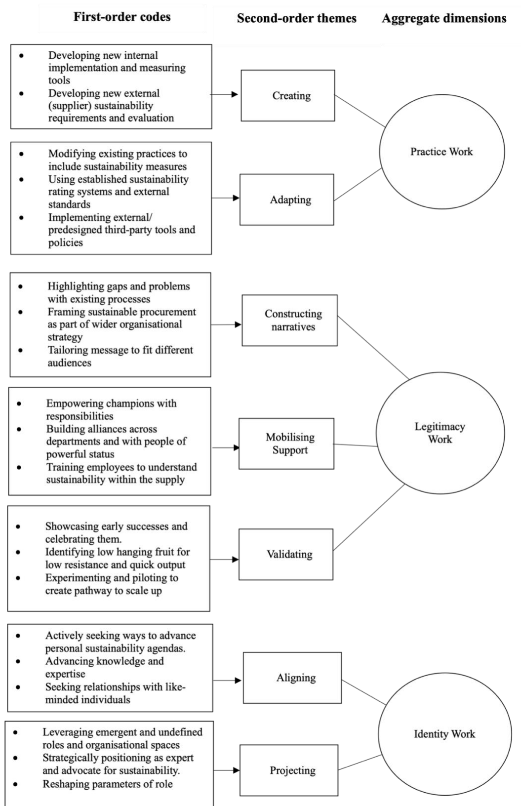
Figure 1- Data Structure
