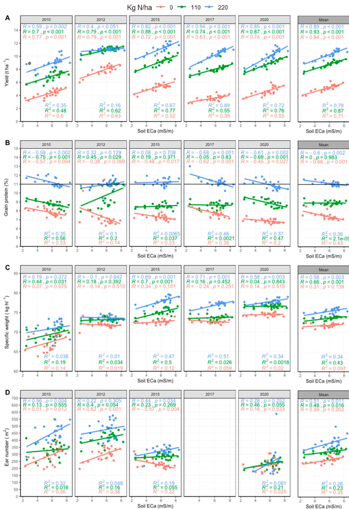
Fig. 4. Linear relationship between plot ECa and wheat performance metrics (2010–2020) and their 5-year means, (A) grain yield, (B) grain protein, where the black line at 11% represents the optimal grain protein for yield, (C) grain specific weight and (D) ear numbers (no ear numbers were recorded 2017). The asterisk (*) in 2010 yield plot represents influential outlier when calculating grain N fertiliser recovery.
