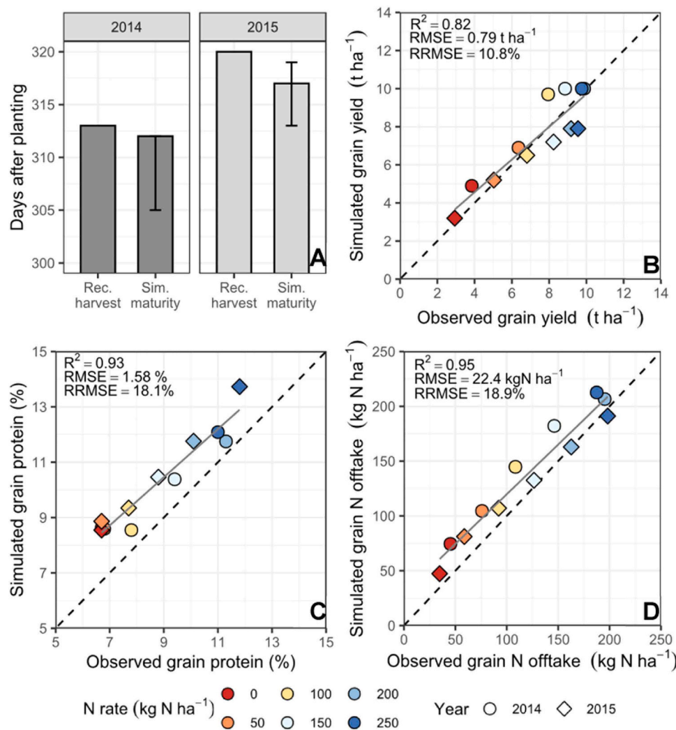
Fig. 6. Comparison of observed and simulated data for wheat performance. (A) Recorded date of harvest compared to simulated maturity date at 200 kg N ha -1 , with error bars representing the maximum and minimum across N rates. (B) Observed yield compared to simulated yield. (C) Simulated grain protein compared to observed grain protein. (D) Observed grain N offtake compared to simulated grain N offtake (Eq. 2).
