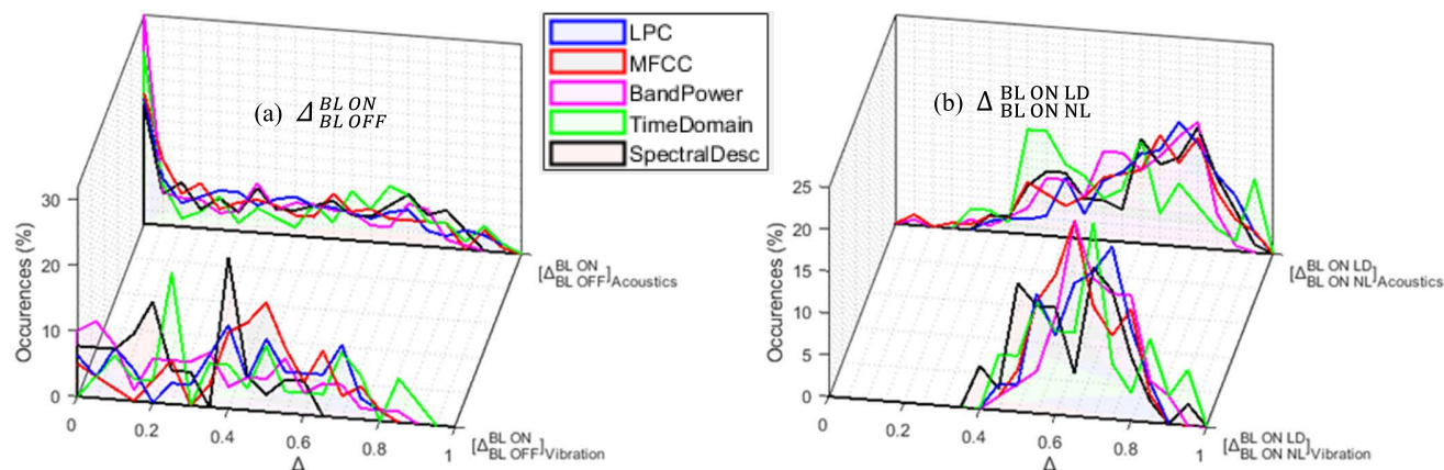
FIGURE 21. Distributions of coefficients of overlap for different categories of acoustic and vibration features.
