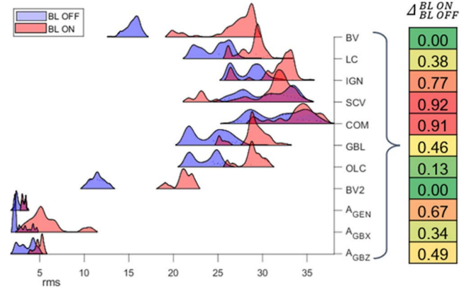
FIGURE 19. Results of \Delta_{BL ON BL OFF}^{BL ON} for RMS feature (Time domain feature category) for all the sensors.
