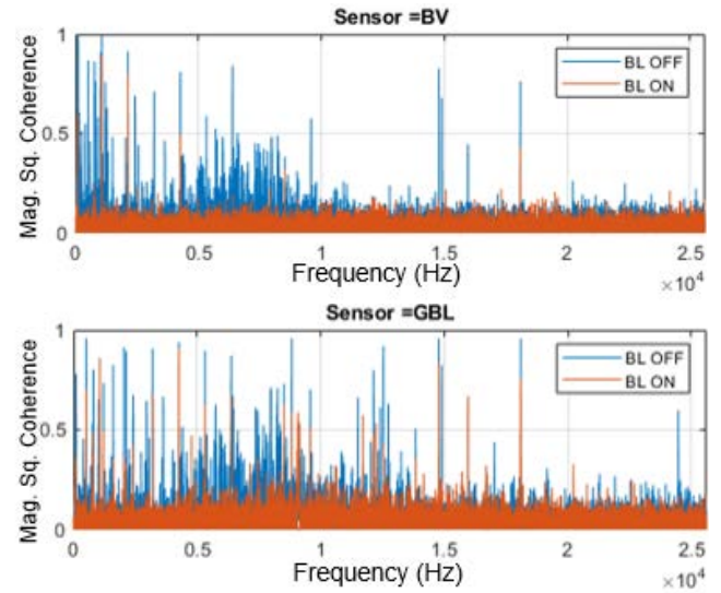
FIGURE 6. Coherence analysis between near-field acoustic sensors and vibration data.
