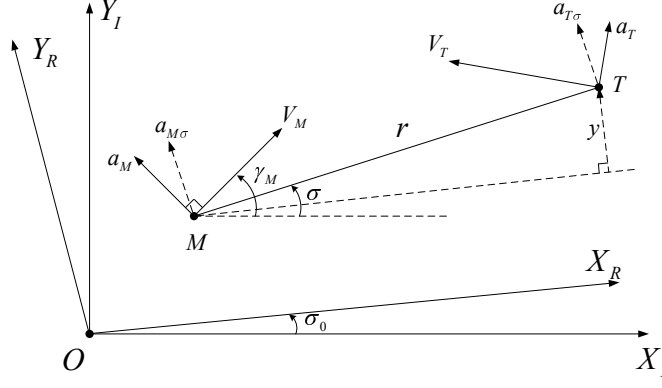
Fig. 1 The homing engagement geometry and parameter definitions.
