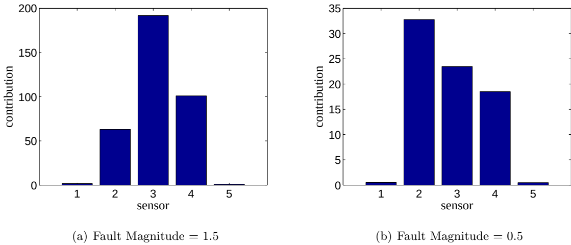
Figure 3: PPCA contribution plot for the multi-sensor fault.
