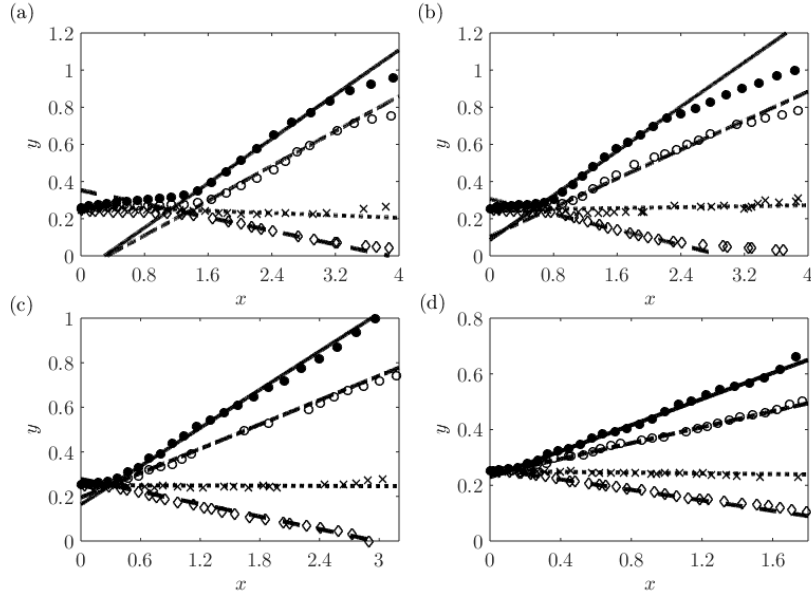
Figure 15: passive scalar iso-curves in PCR for Sc=1 . \Phi = 0.1 , data ( \bullet ), regression (-). \Phi = 0.4 , data ( \circ ), regression (-.-). \Phi = 0.7 , data ( \times ), regression (...). \Phi = 0.9 , data ( \diamond ), regression (--). (a) Re = 5000 ; (b) Re = 10,000 ; (c) Re = 20,000 ; (d) Re = 40,000 .
