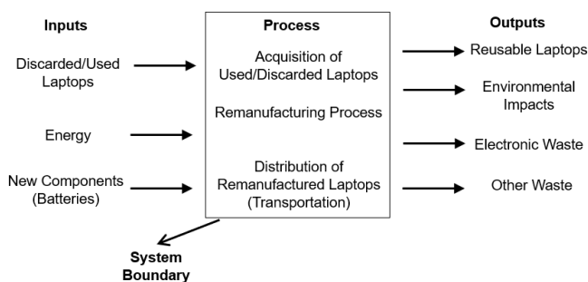
Fig. 3. Product system boundary.
