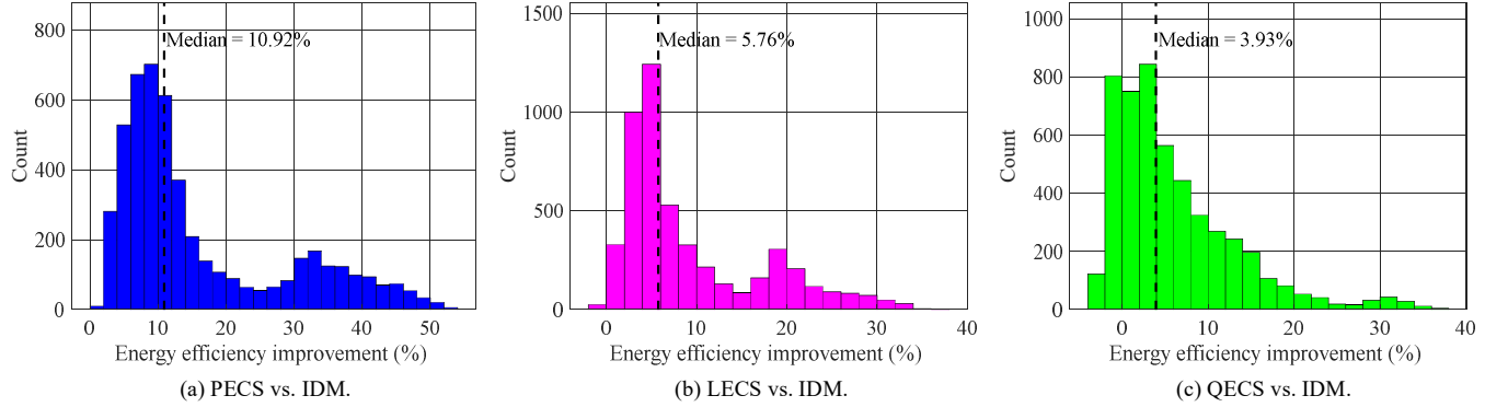
Fig. 13. Energy efficiency improvement of different strategies during 5,000 stochastic simulations.
