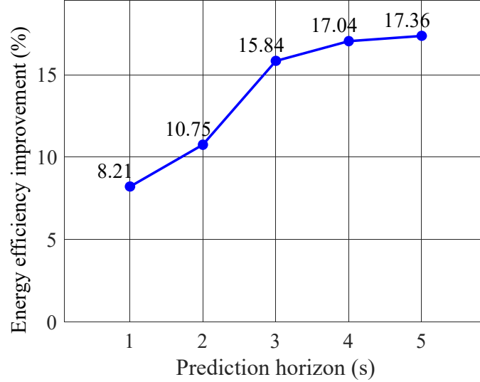
Fig. 9. Average performance analysis of the PECS under different prediction horizons.
