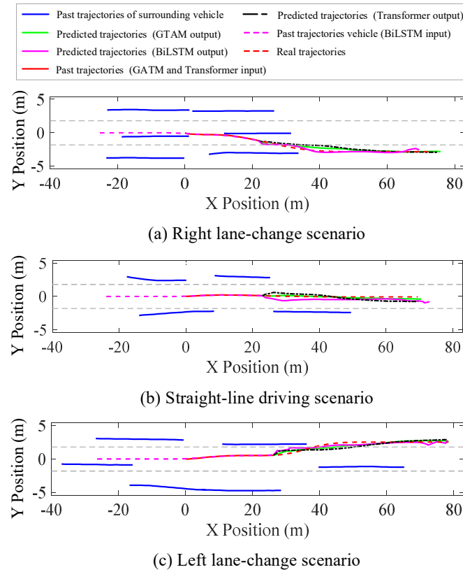
Fig. 11. Lane-changing trajectory schematic.
