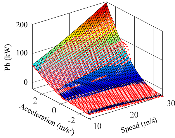
Fig. 7. The fitting result of battery power.
