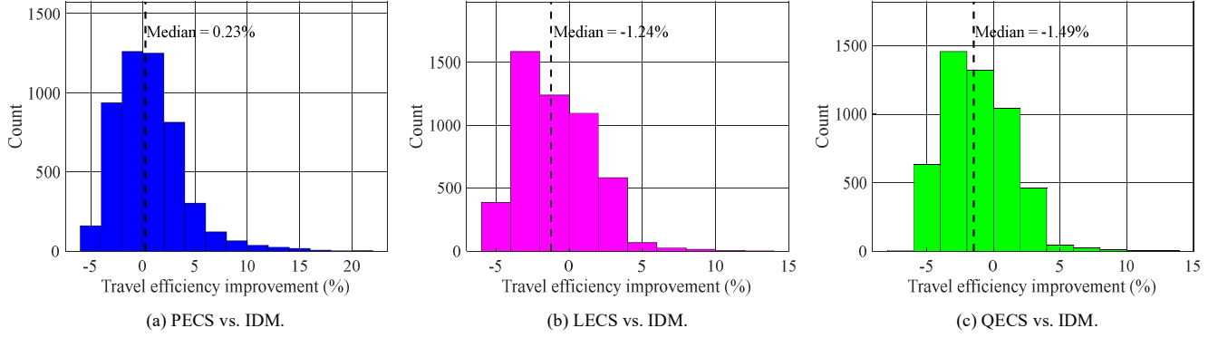
Fig. 14. Travel efficiency improvement of different strategies during 5,000 stochastic simulations.
