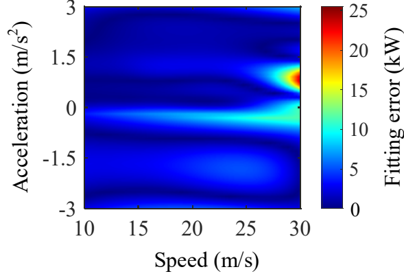
Fig. 8. The fitting error of battery power.
