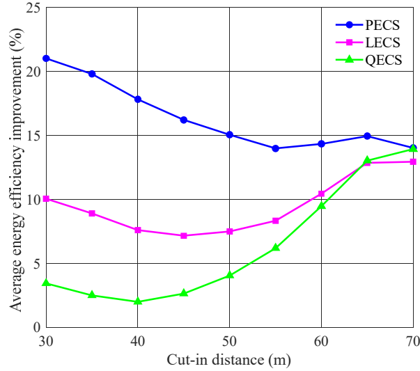
Fig. 15. Distribution of energy efficiency improvement dependence on cut-in distance.
