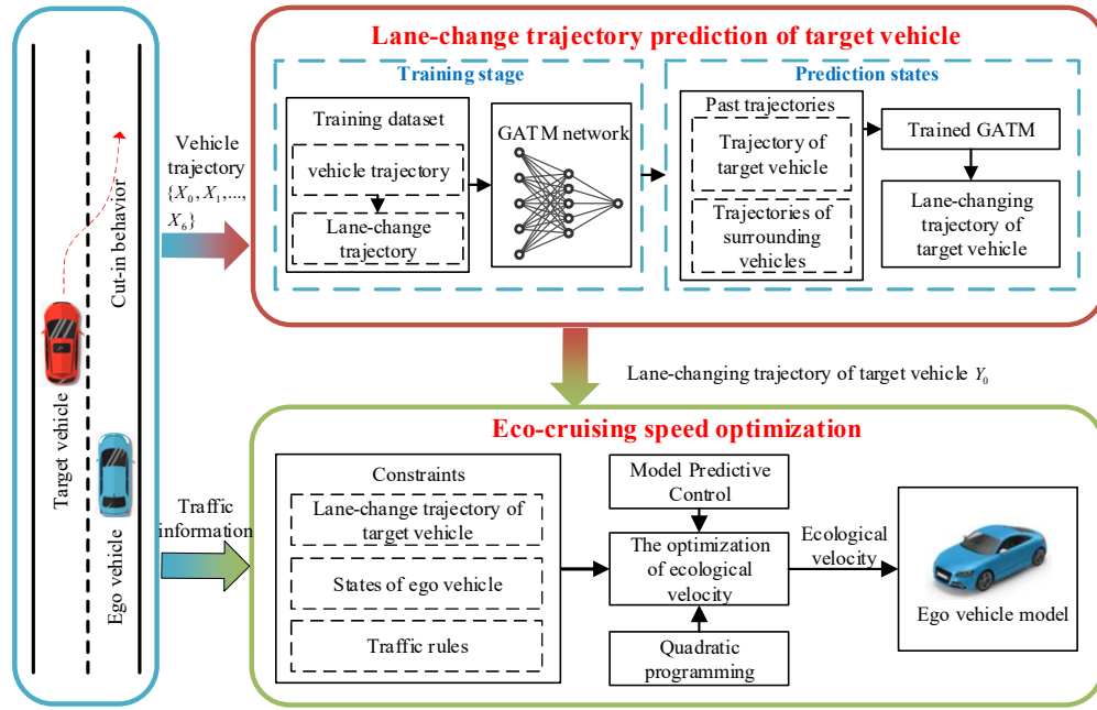
Fig. 3. The hierarchical control scheme of the PECS.
