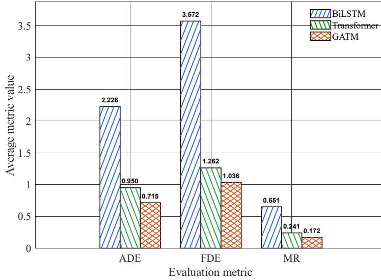
Fig. 10. Comparative experiments on the test set.
