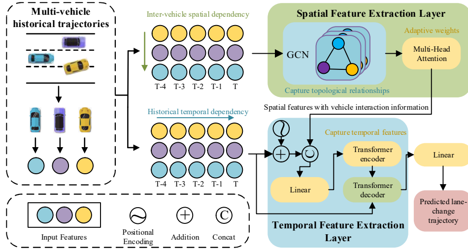
Fig. 4. Structure diagram of GATM vehicle trajectory prediction model.
