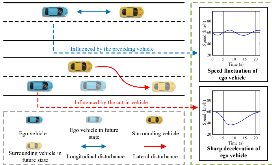
Fig. 1. The stochastic disturbances from surrounding vehicles.
