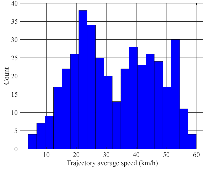
Fig. 6. Speed distribution of the trajectories.
