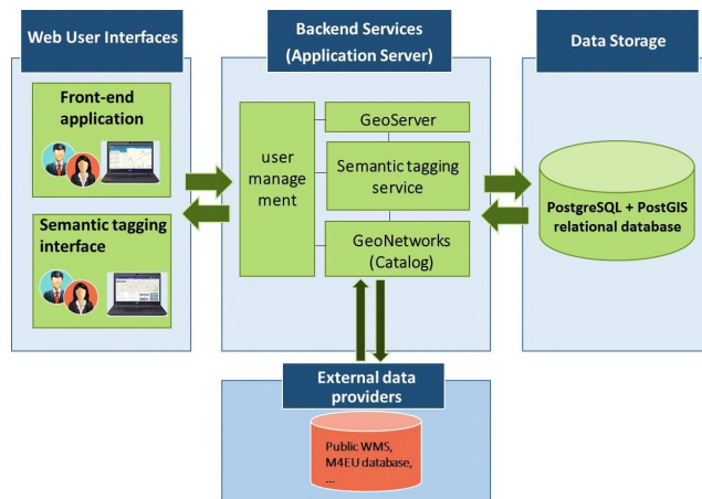
Fig. 6. High level components of Smart Ground Platform
