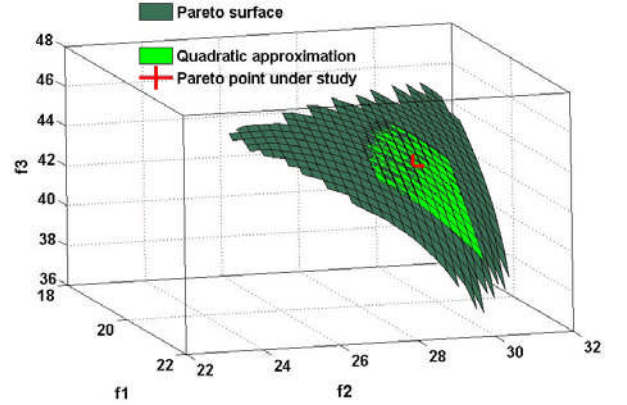
Figure 2: Quadratic approximation
