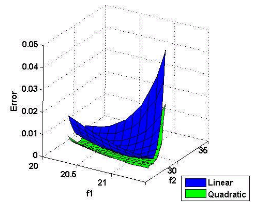
Figure 3: Error in predicting f_3
