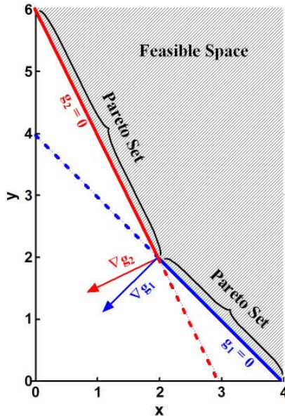
Figure 4: Example 2 – Design space / Pareto set
