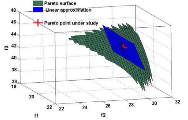
Figure 1: Linear Approximation
