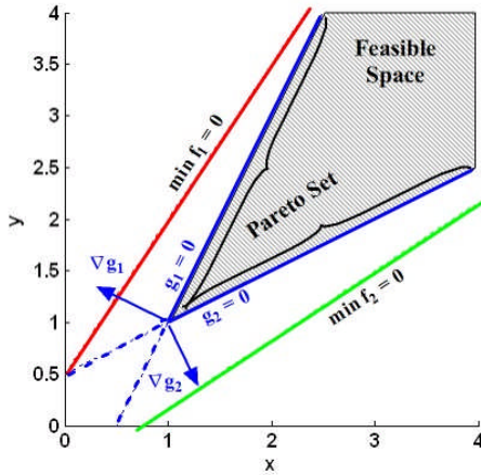
Figure 6: Example 3 – Design space / Pareto set
