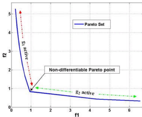
Figure 7: Example 3 – Objective space / Pareto set
