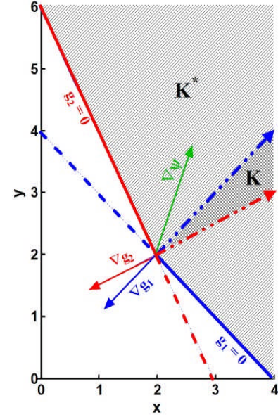
Figure 5: Example 2 - Relative position of the tangent cone and its polar at a non-differentiable Pareto point
