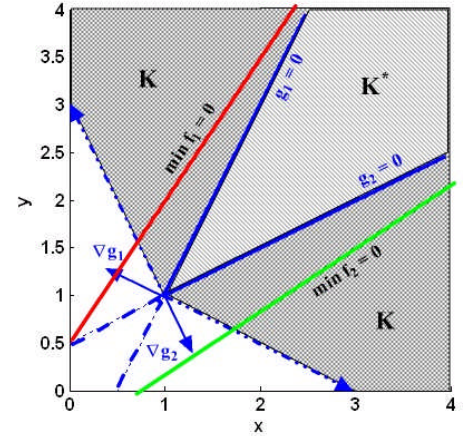
Figure 8: Example 3 - Relative position of the tangent cone and its polar at a non-differentiable Pareto point
