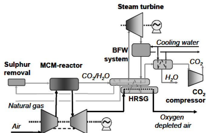
Figure 7: AZEP cycle schematic [17]
