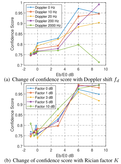
FIGURE 11. Confidence scores in unknown environments.
