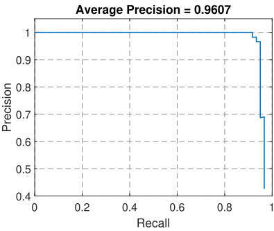
FIGURE 9. Precision-recall curve for the proposed identification framework in the training phase.
