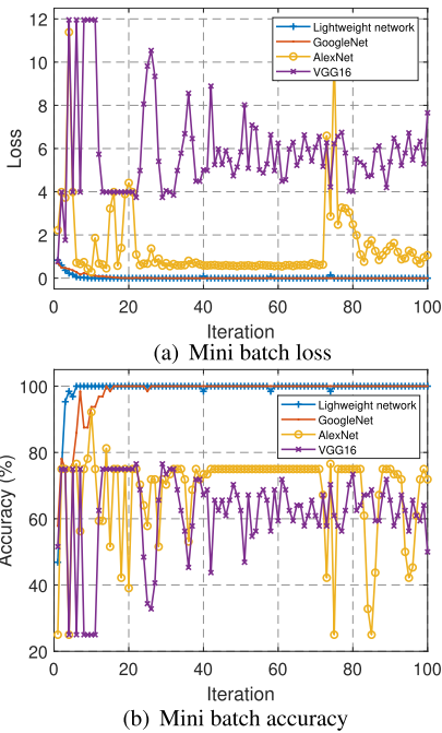
FIGURE 10. Comparison of loss and accuracy for popular deep neural networks.
