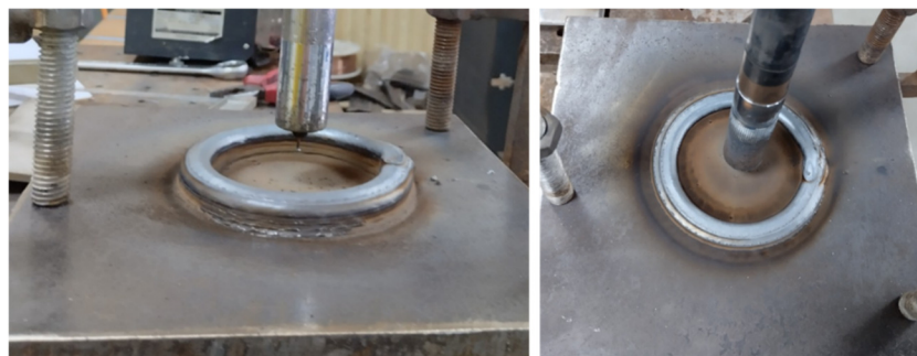
Fig. 6 Multi-bead multi-layer cylindric part
