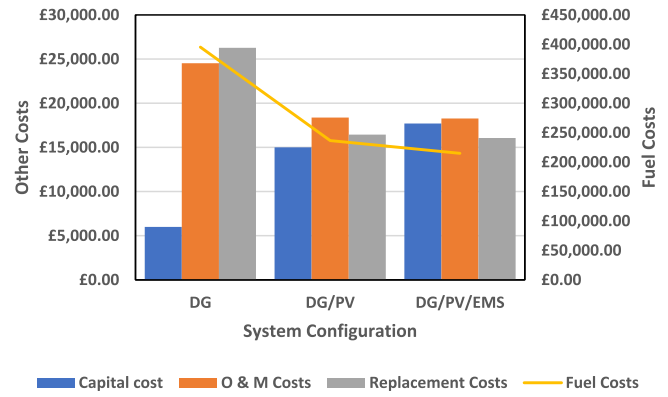
Fig. 8. Cost comparison of DG, DG/PV, and DG/PV/IEMS configurations.
