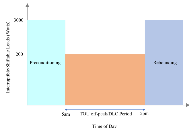
Fig. 6. Demand load control/time-of-use program.
