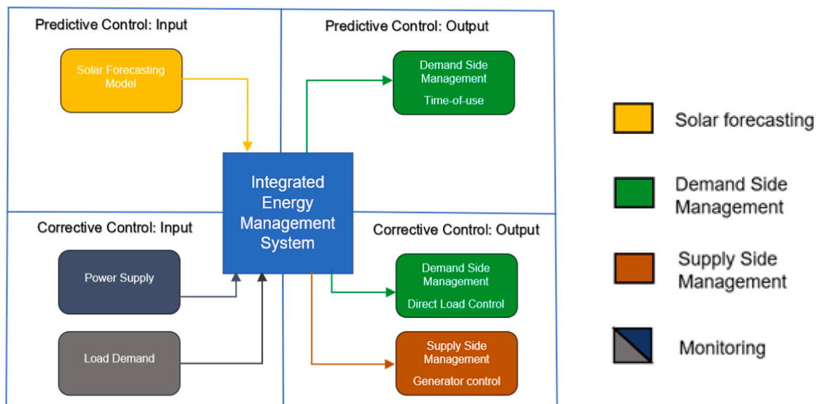
Fig. 1. Proposed integrated energy management system framework.
