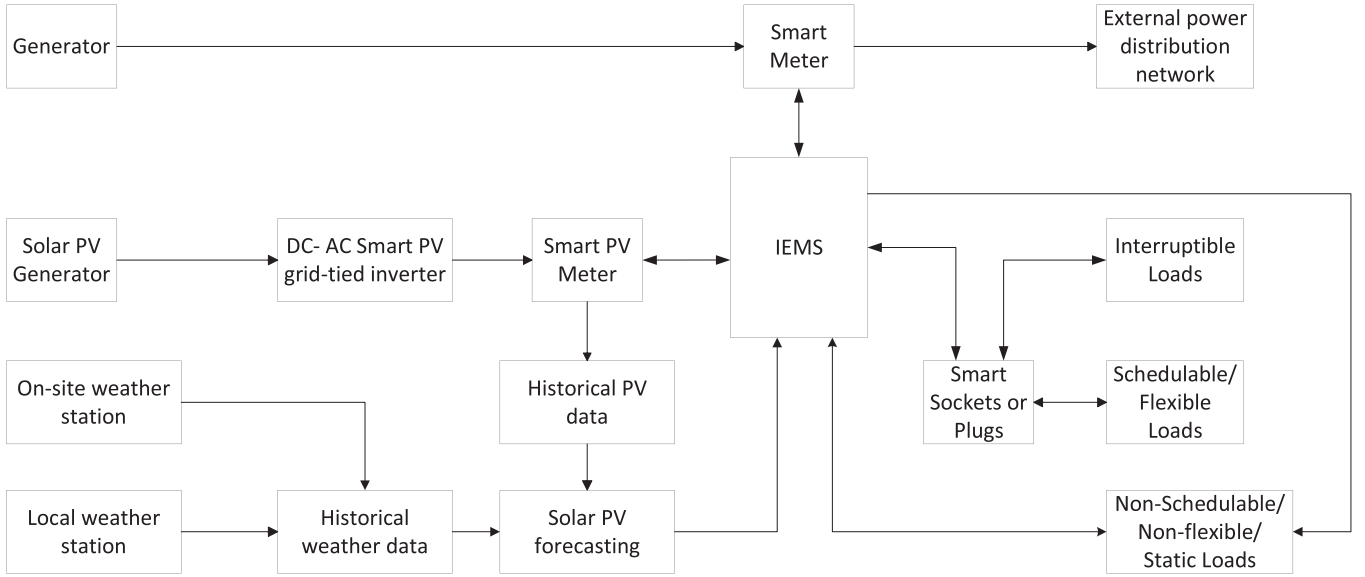
Fig. 2. Block diagram of proposed IEMS.
