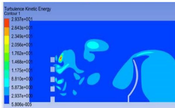
FIGURE 2a. Turbulent kinetic energy for a porous barrier
