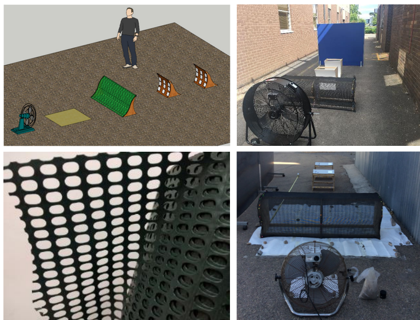
FIGURE 7. Outdoor testing of small dust barriers - with the following details: Schematic (upper left), Porous mesh (lower left), Cranfield experiment (upper right), PSA experiment (lower right)
