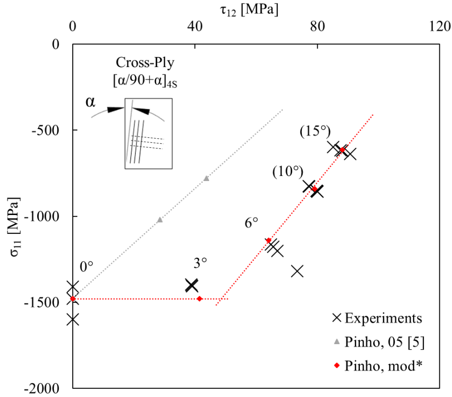
452 Figure 14. Longitudinal ( \sigma_{11} ) vs shear ( \tau_{12} ) stress at failure for the 0, 3, 6, 10 and 15° CP Cub 453 specimens, extracted using CLT. Brackets on 10 and 15° results indicate that a correcting factor 454 has been applied to correct for fibre rotation. Grey markers indicate predicted failure stresses for 455 each case using the fibre kinking theory proposed by Pinho [5] and red markers indicate predictions 456 using the proposed modification. Numerical predictions were only calculated for the five off-axis 457 loading cases, dotted trend lines are extrapolated from these results.
