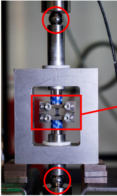
(a) Alignment fixture
