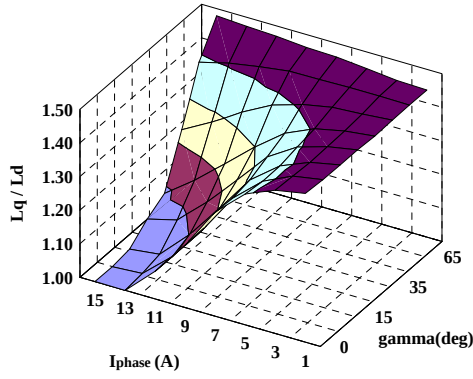
Figure 13: L_q/L_d as a function of phase current and advanced commutation angle.
