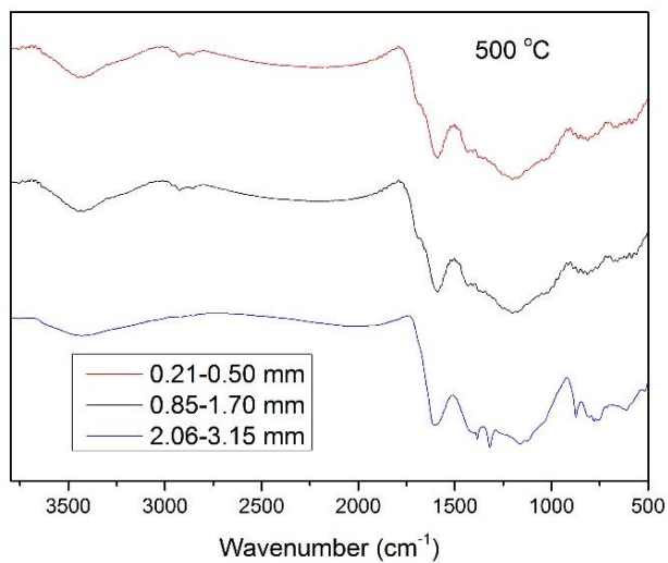
Figure SM-4. FTIR of chars produced from BWC of different particle size at different temperatures.
