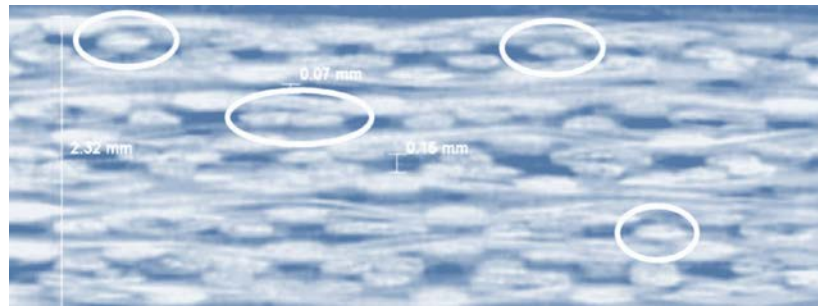
Figure 1. X-ray tomography image (right) [14,15] showing the lenticular shape of yarn in a cured composites (example woven composites satin weave ACG SL246/40)
