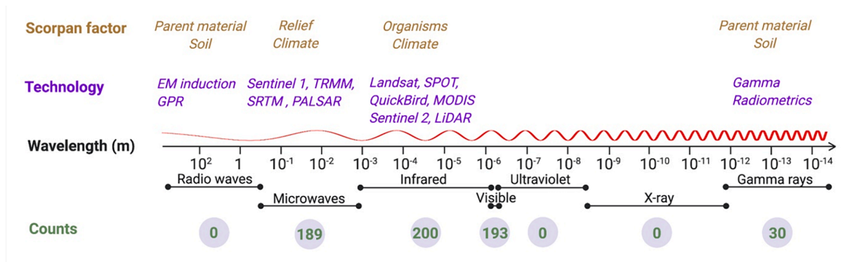
Fig. 11. Sensing techniques and their relevance to Scropan factors. Counts indicate the frequency of different bands used as environmental covariates.
