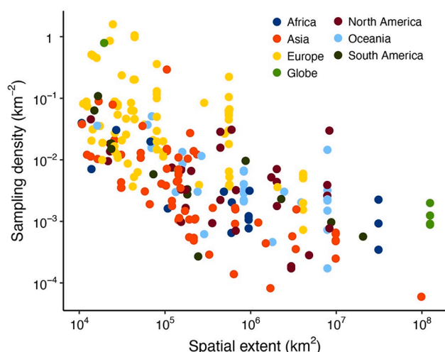
Fig. 3. Trend between spatial extent and sampling density (number of soil sampling sites \text{km}^{-2} ).
