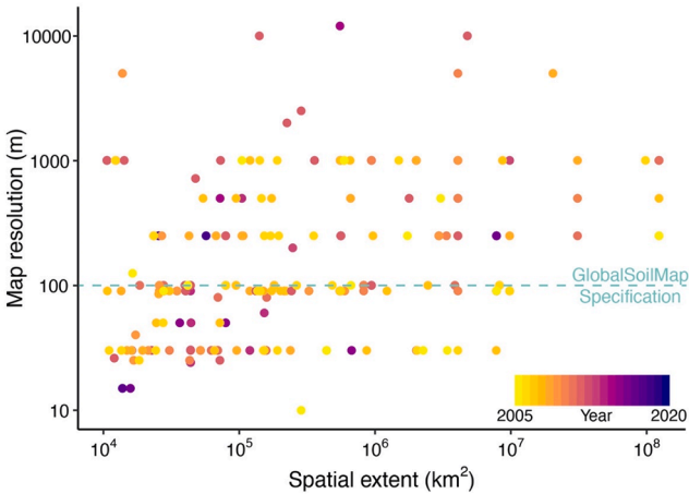
Fig. 7. Relationship between map resolution and spatial extent.
