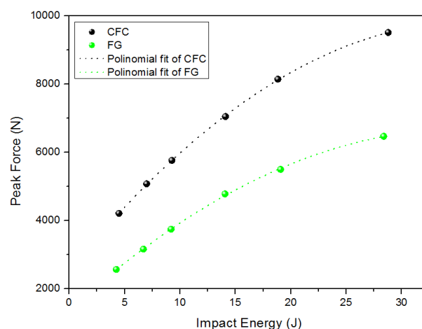
Figure 7. Peak force as a function of the impact energy for the carbon fibers (black) and glass fibers (green).
