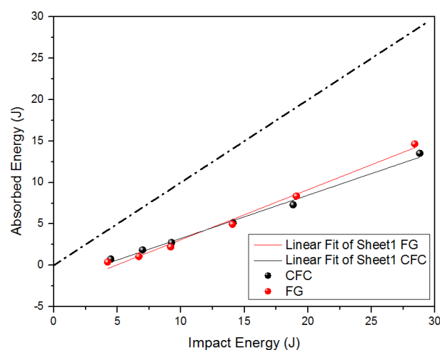
Figure 6. Energy profile with the equal energy curve.
