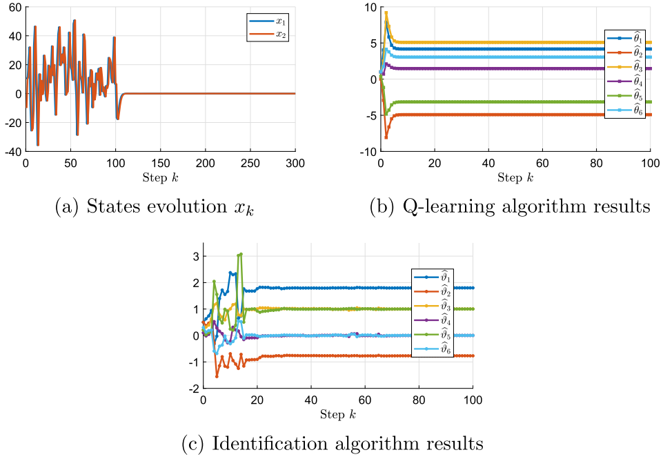
Fig. 4. Neocortex results.
