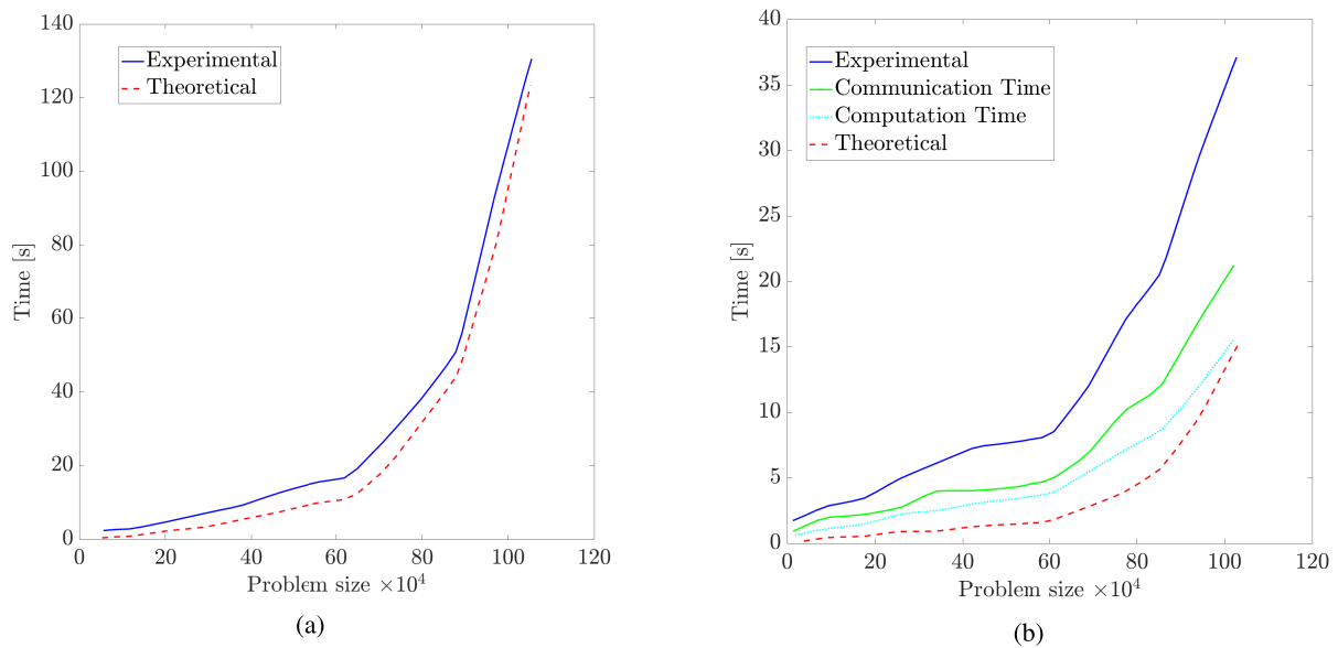
FIGURE 11. Comparison of the execution time of the hybrid algorithm developed in [17] over: (a) a single machine, or (b) a parallel cloud. For each curve, a theoretical computational time is also provided. Panel (b) also explicitly breaks down the overall experimental time into computation and communication times (data source: [17]).
