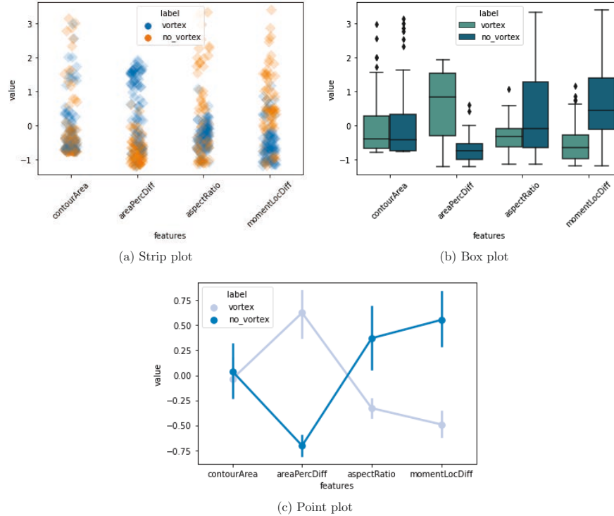
Figure 11 Feature distributions using EDA.
