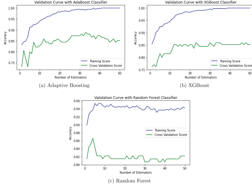
Figure 14 Training and validation curves of individual classifiers.
