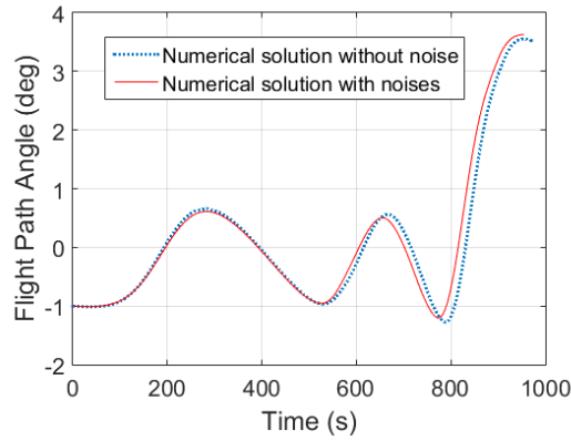
Figure 20: Flight path angle vs time
