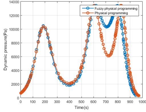
Figure 16: Dynamic pressure for different objective function
