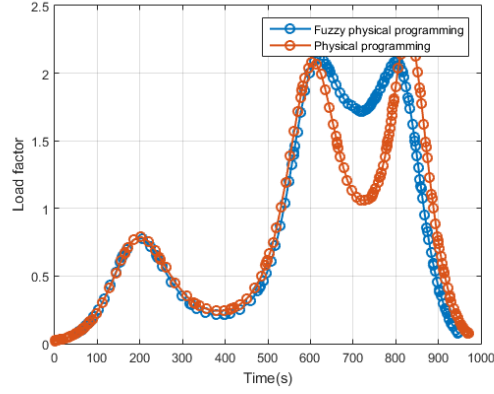
Figure 14: Load factor for different objective function
