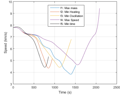
Figure 4: Speed for different objective function
