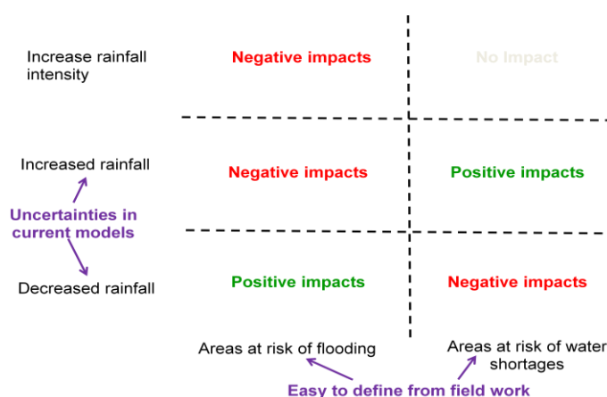
Figure 3: Impacts of climate change on flood and drought prone areas
