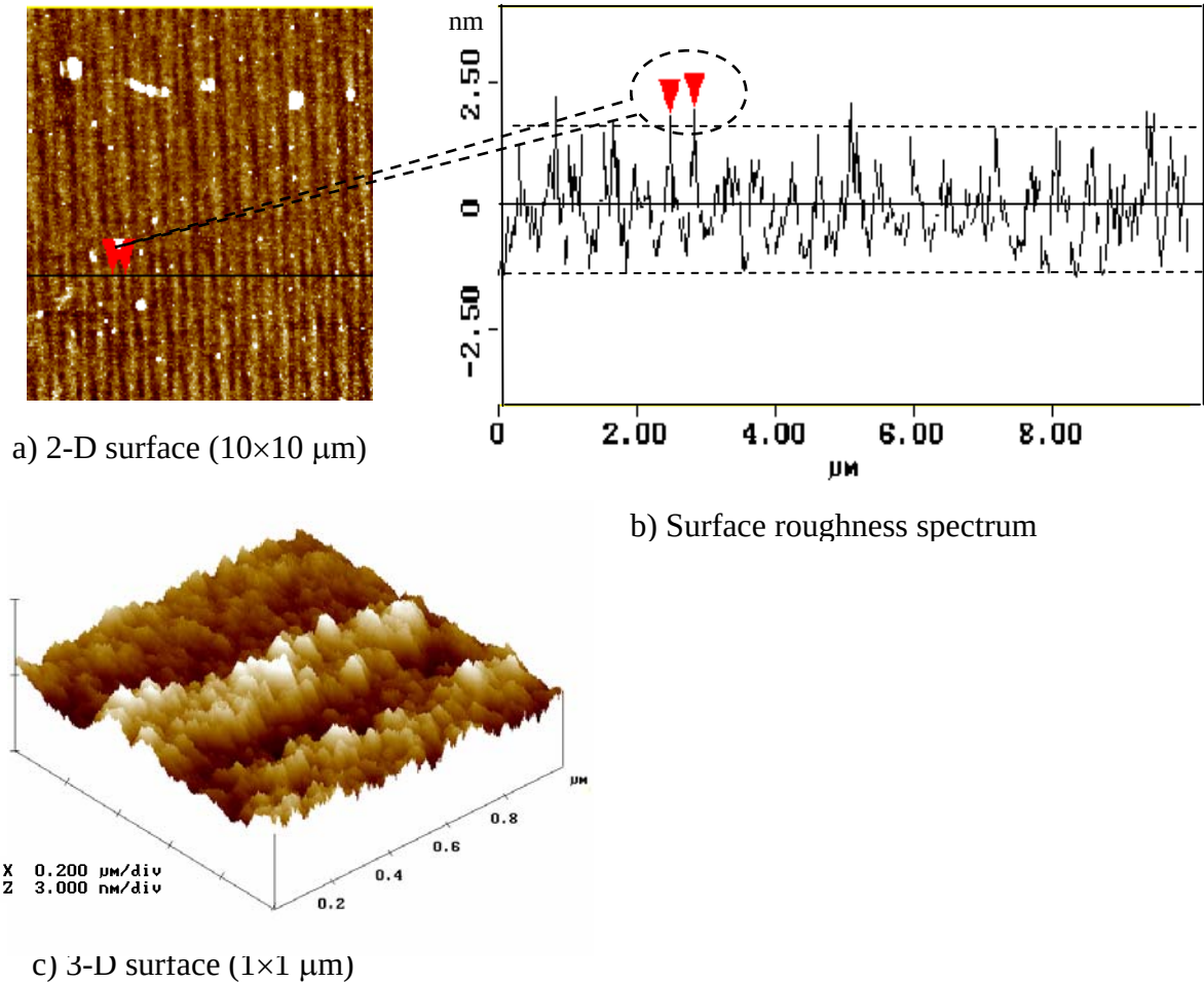
Fig. 8 AFM image of irradiated Ge-B codoped fibre surface (FBG inscription condition: 266nm laser, 2.8 W/cm 2 pulse average density)
