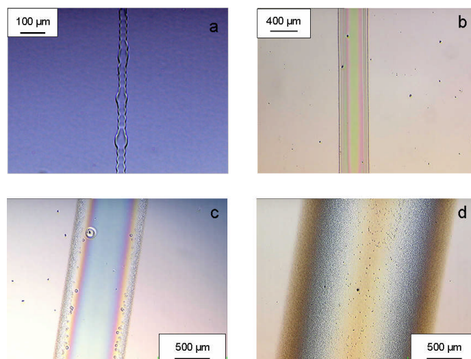
Fig. 5. EHDA deposition of 0.6M PZT sol into lines of differing widths. At narrow widths (a; 50 \mu\text{m} ) the formation of the line from adjacent droplets is noticeable. At larger widths (b; 400 \mu\text{m} ), the lines are smooth-walled. After a certain line width the film deposition decreases in quality (c), until there is no continuous film present (d).
