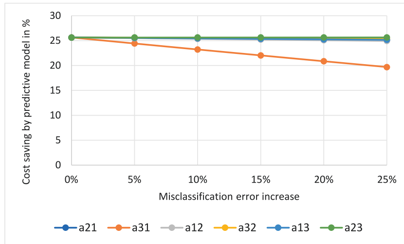
Fig. 7. Cost saving percentage vs predictive model classification errors increasement.
