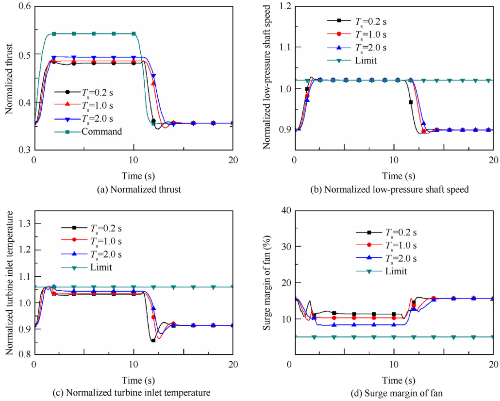
Fig. 4 Parameter responses with different time constants.
