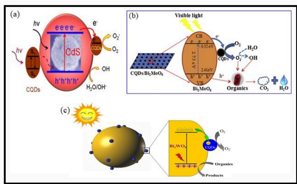
Fig.9. Schematic representation of charge transfer mechanism of (a) CQDs/CdS, (b) CQDs/ Bi_2MoO_6 (c) CQDs/ Bi_2WO_6 narrow band gap photocatalyst composite (With permission from Elsevier, license number 4517510659557, 4474120216249, 4517511222302).
