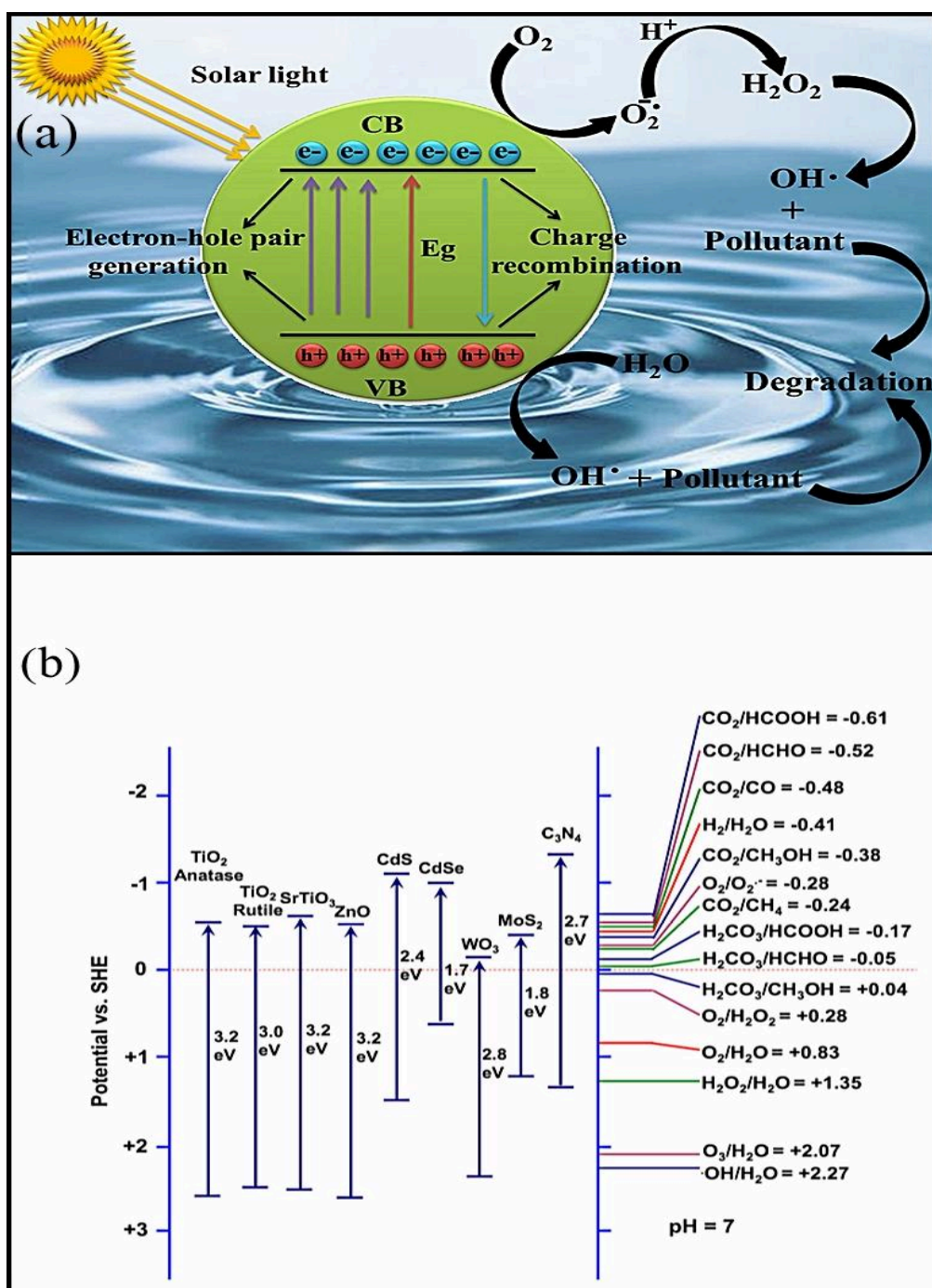
Fig. 2. (a) Basic photocatalytic mechanism of a photocatalyst depicting degradation of organic pollutants present in water (With permission from Elsevier, license number 4471830715641)
