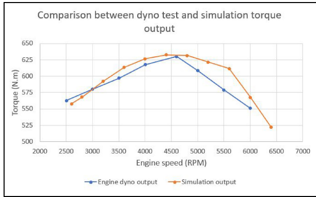
Figure 4. Torque curve comparison between AVL Boost TM model and LT1 engine dyno test. 26
