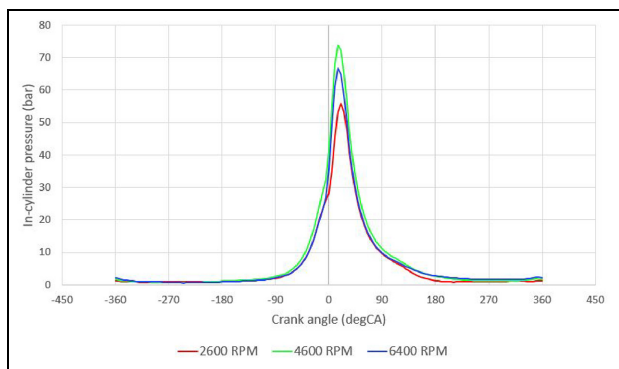
Figure 5. Cylinder pressure traces in crank angle domain at 2600, 4600 and 6400 rpm.
