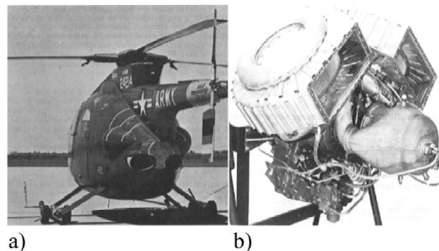
Figure 1: (a). Modified YOH-6A helicopter (AUM=998 kg); (b). T63 helicopter turboshaft engine with twin tubular "bolt-on" recuperator modules, reproduced from (7) .
