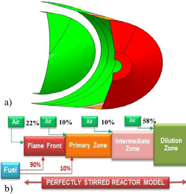
Figure 4: a). Combustion chamber of reference Rolls-Royce Allison 250-C20B engine; b) Combustor zones and reactor models assumed for NO x modelling of rotorcraft combustor.
