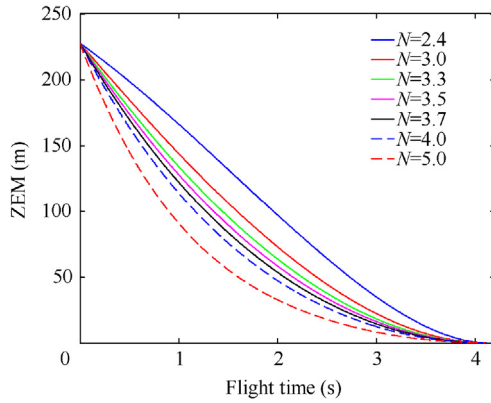
Fig. 10 Zero-miss-effort (Initial states 1 and constant target maneuver).
