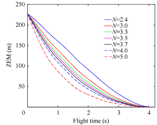
Fig. 22 Zero-miss-effort (Initial states 1 and sinusoidal target maneuver).
