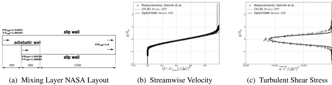
Figure 1: Mixing Layer
