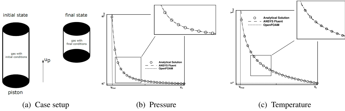
Figure 8: Isentropic Compression
