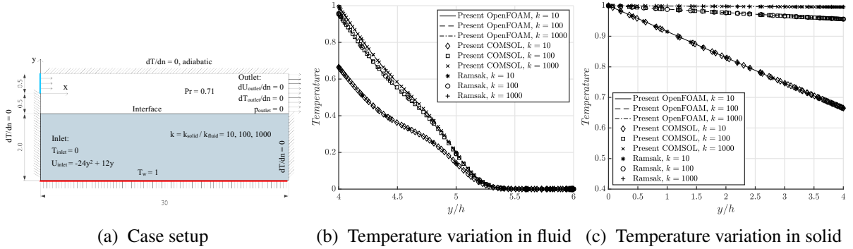
Figure 9: Conjugate Heat Transfer at x = 6h
