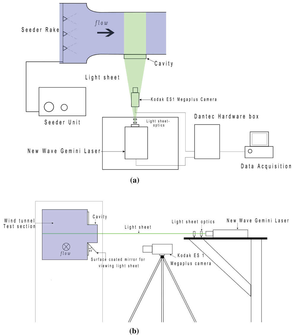
Fig. 6 Schematic of the PIV set-up. a Top view. b Side view
