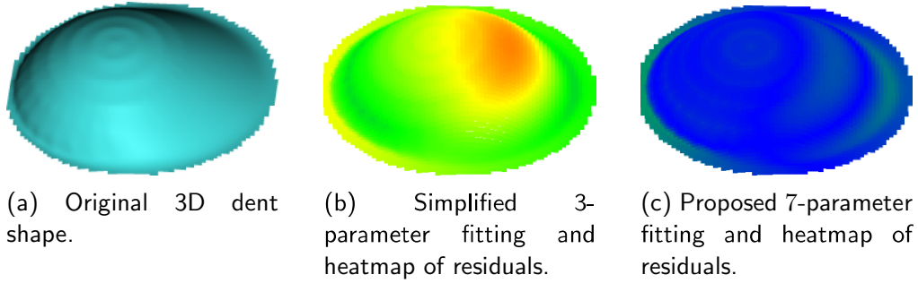
Figure 8: Dent obtained from a 45° collision and residual heatmaps (blue = 0 mm, red = 1 mm mm). The proposed model is capable to follow the natural dent shape and the MAE is reduced by an order of magnitude.
