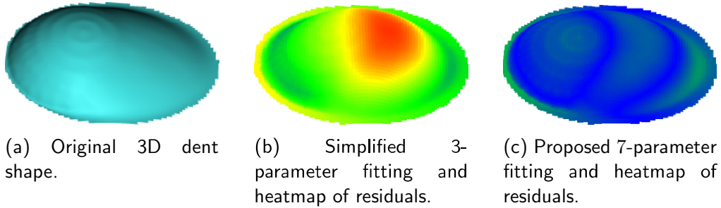
Figure 9: Dent obtained from a 60° collision and residual heatmaps (blue = 0 mm, red = 1 mm mm). Also in this case the MAE is greatly reduced.
