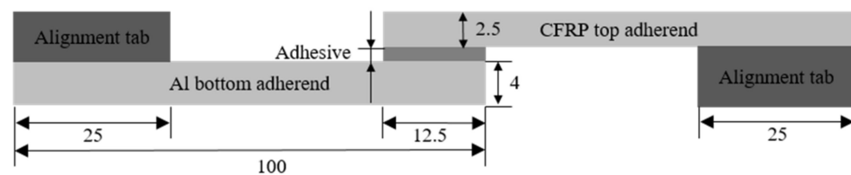
Figure 2. Geometry and dimensions of single lap joint (SLJ) specimens following the guidance of the BS EN 1465:2009 standard. The width of the single lap joint was 25 mm (polyurethane joint design shown; units in mm).
