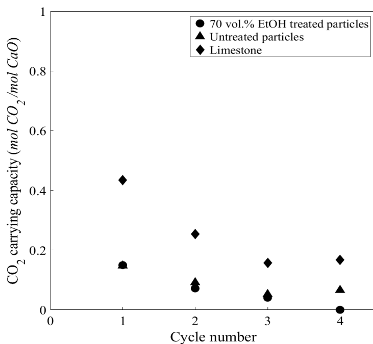
Figure 4 – CO 2 carbonation carrying capacity over 4 calcium looping cycles, of 70 vol.% EtOH/water treated and untreated particles (400 – 600 µm) which were composed of calcined limestone, a calcium aluminate cementitious binder and flour as a pore forming spacer, and natural limestone for baseline comparison. Conducted within fluidised bed reactor, carbonation performed in 15 vol.% CO 2 and 85
