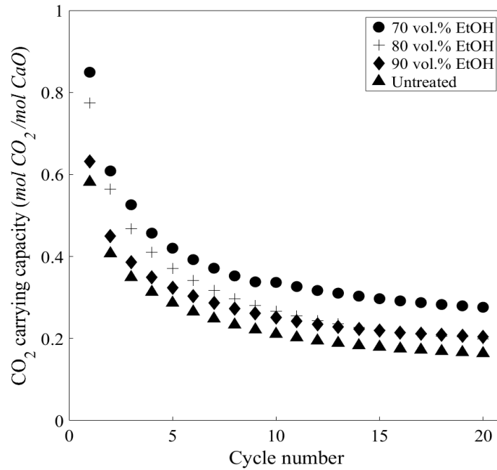
Figure 2 – CO 2 carrying capacity over 20 calcium looping cycles, of EtOH/water pre-treated particles (300 – 500 \mu\text{m} ) with a calcium aluminate cementitious binder and flour as a biomass pore forming spacer. Conducted within an atmospheric TGA, carbonation performed at 650 ^{\circ}\text{C} for 20 minutes and calcination at 950 ^{\circ}\text{C} for 1 minute. The CO 2 partial pressure was ramped between the carbonation and calcination conditions to prevent undesired early calcination [25].
