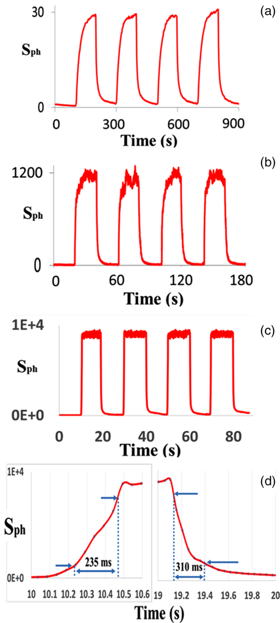
FIGURE 5 The photoresponse characteristics of the (a) ZNWA-based, (b) single ZNW-based and (c) ZNB-based PDs. (d) The corresponding response and recovery times of the ZNB-based PDs. PD, photodetector.
