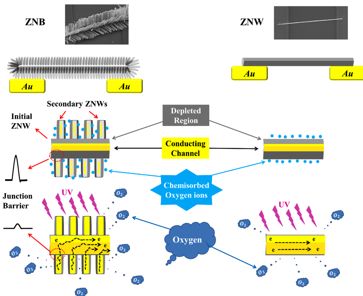
FIGURE 6 Schematic diagram showing the carrier generation and transportation process in the ZNW-based versus the ZNB-based UV PDs. UV, ultraviolet.
