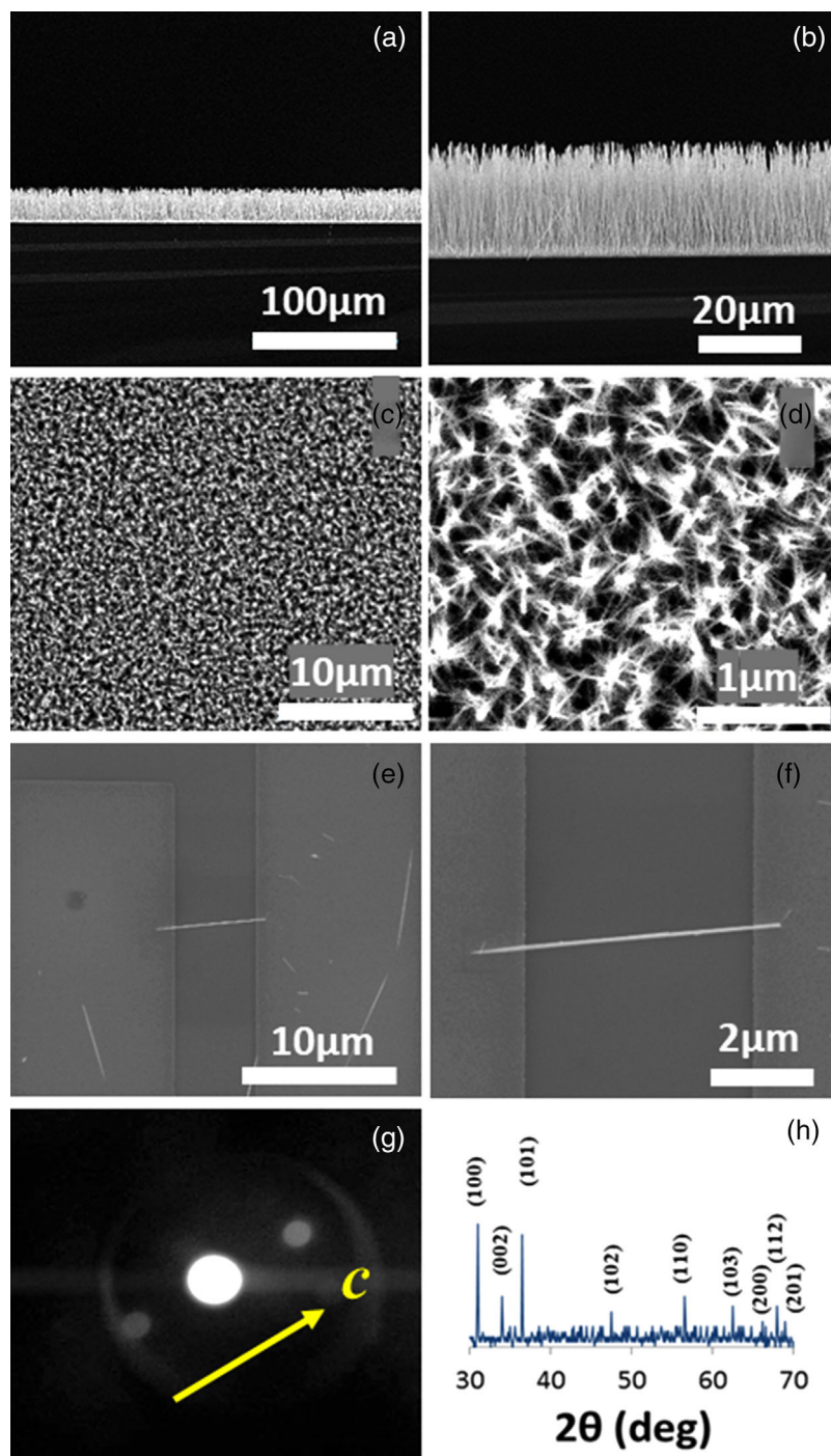
FIGURE 1 (a) Low-magnification side-view SEM image, (b) high-magnification side-view SEM image, (c) low-magnification top-view SEM image, and (d) high-magnification top-view SEM image of an array of ZNWs. (e) Low-magnification SEM image and (f) high-magnification SEM image of a single ZNW. (g) The corresponding SAED pattern for the ZNWs and (h) the XRD pattern of the ZNWs. SAED, selected areas of electron diffraction; SEM, scanning electron microscopy; XRD, X-ray diffraction; ZNW, zinc oxide nanowires.
