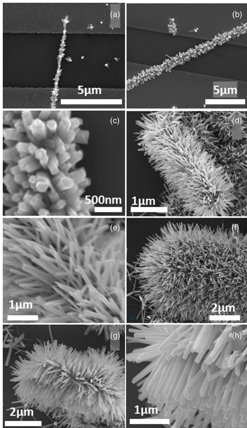
FIGURE 4 (a) SEM image of a ZNB bearing a low density of secondary ZNWs. (b) SEM image of a ZNB bearing a high density of secondary ZNWs. (c) High-magnification SEM image of the high-density secondary ZNWs. (d) SEM images of a ZNB bearing a high density of long secondary ZNWs. (e) High-magnification SEM image of the secondary ZNWs. (f, g) SEM images of ZNBs grown from initial ZNPs with a high secondary ZNW density. (h) A high magnification SEM image of the highly dense secondary ZNWs
