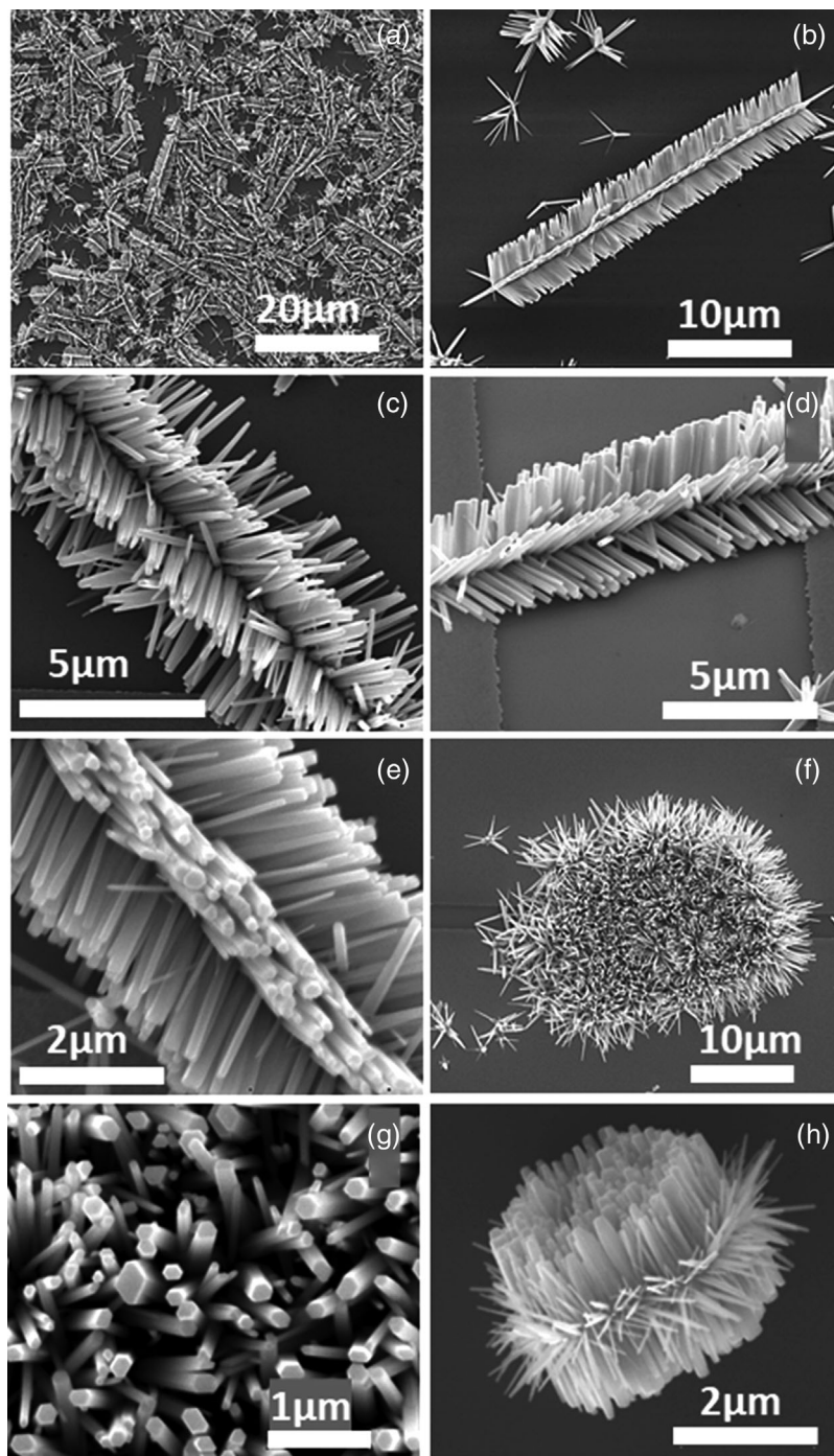
FIGURE 3 (a) SEM image showing numerous ZNBs grown from the initial ZNWs. (b) SEM image of a single ZNB. (c) SEM image of a ZNB connecting two gold electrodes. (d) High-magnification SEM image of a single ZNB. (e) High-magnification SEM image of the secondary ZNWs. (f) Top-view SEM image of a ZNB grown from an initial ZNP. (g) High-magnification top-view SEM image of the ZNB. (h) Tilted-view SEM image of a ZNB. ZNB, zinc oxide nanobrushes.
