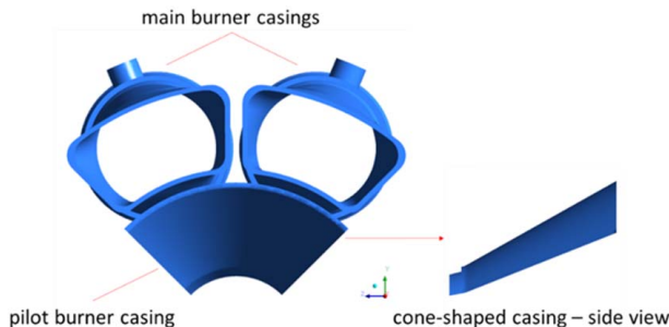
Fig. 2 Main burners casing, pilot burner, and side view of the cone-shaped pilot casing
