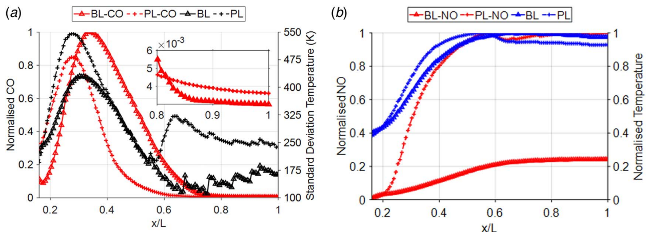
Fig. 13 Pollutants, their standard deviation temperature, and normalized mass-average temperature for baseload and part-load: (a) CO concentration and (b) NO concentration
