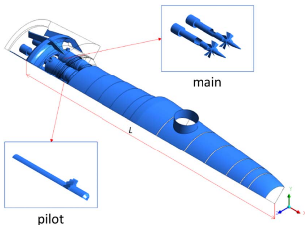
Fig. 3 The quarter section model of the combustor
