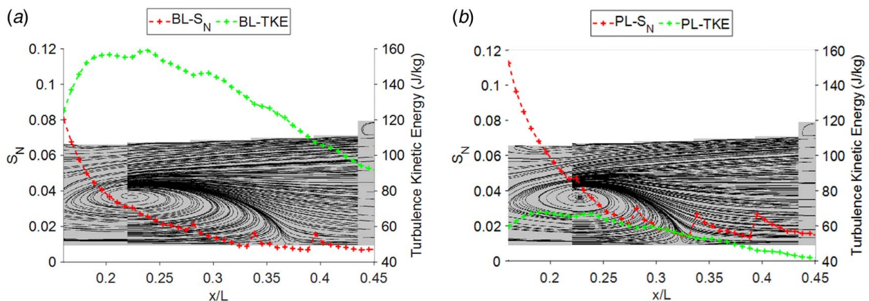
Fig. 11 Recirculation zone profiles of normalized unmixedness and mass-averaged TKE: (a) baseload and (b) part-load
