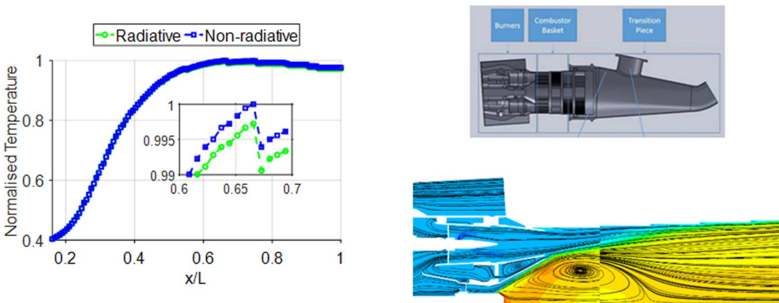
Fig. 7 Axially averaged temperature across the combustor (left) 3D model and contour of the temperature (right)
