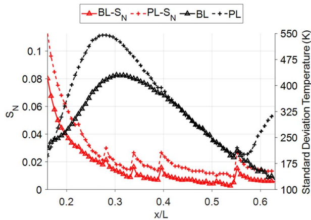
Fig. 12 Unmixedness and standard deviation temperature at baseload and part-load
