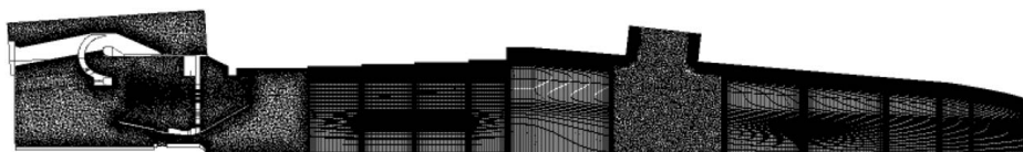
Fig. 4 Reduced model computational mesh
