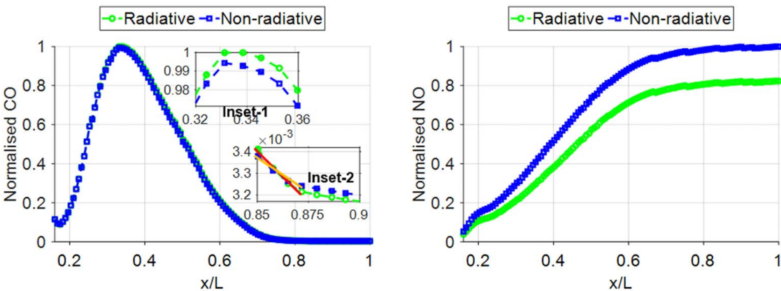
Fig. 8 Axial mass-averaged CO and NO for radiative and non-radiative cases
