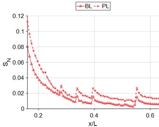
Fig. 10 Normalized unmixedness across the combustor—baseload and part-load
