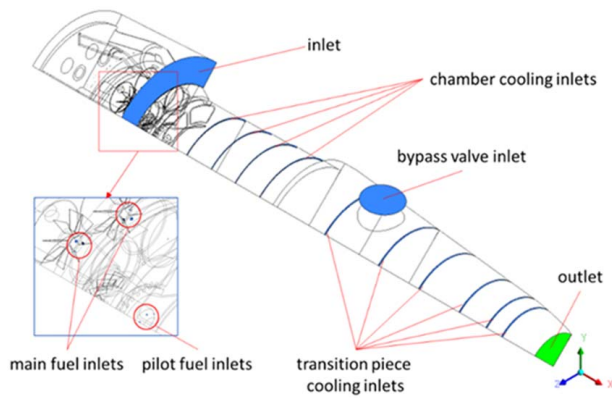
Fig. 5 Boundary conditions on the model
