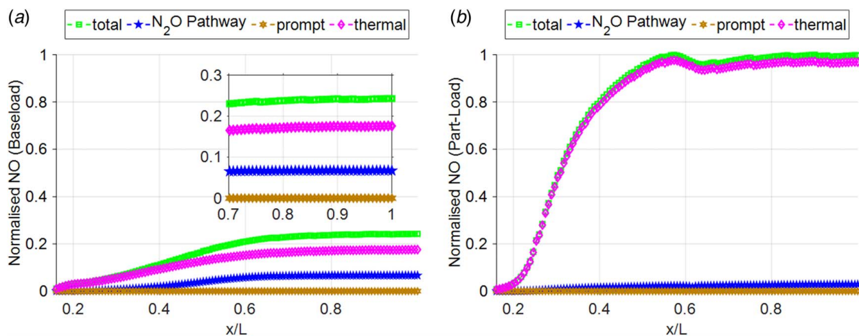
Fig. 14 Contribution of different formation pathways to the total NO: (a) baseload (b) part-load
