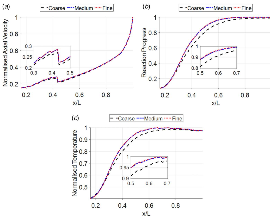
Fig. 15 From left-to-right: (a) mass-averaged velocity axial, (b) mass-averaged reaction progress, and (c) mass-averaged temperature
