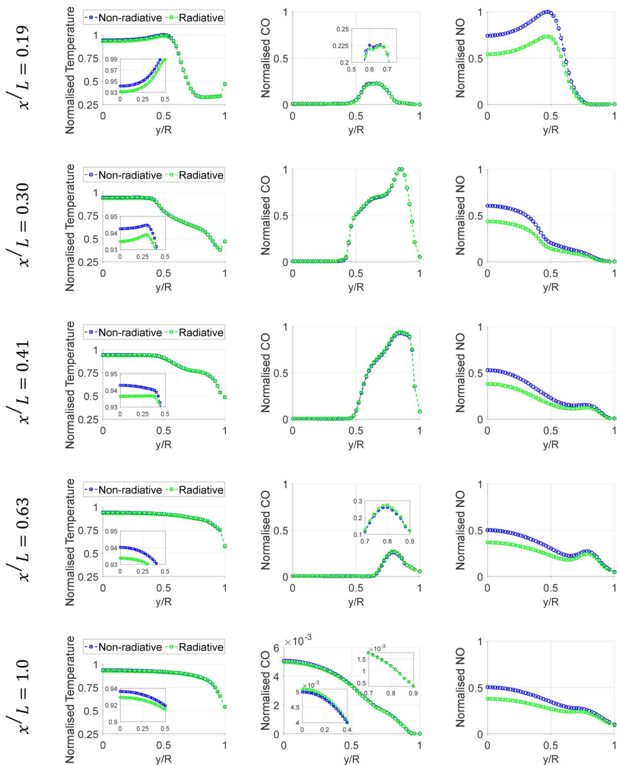
Fig. 9 Radial averaged temperature, CO and NO at normalized axial positions for radiative and non-radiative cases
