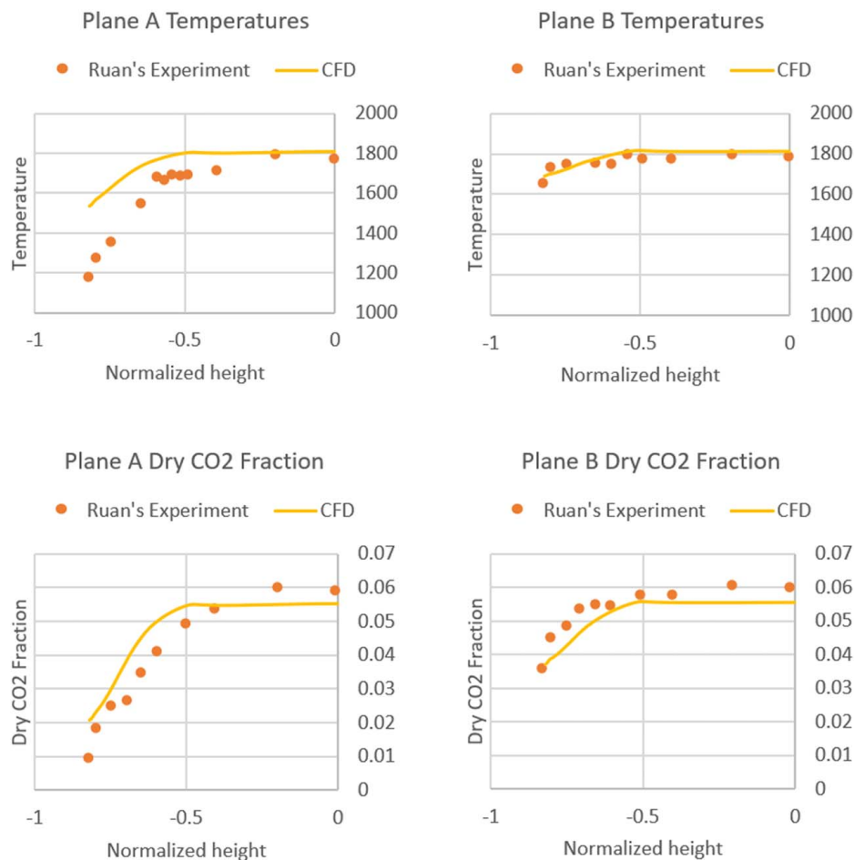
Fig. 6 Radial profiles of temperature (top) and mass fractions of CO 2 (bottom) at planes A and B
