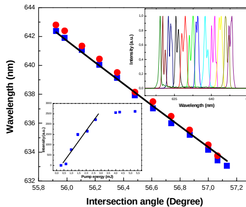
Fig. 2. Output wavelengths as a function of the internal intersection angle \theta_{in} in LCP:LCP pumping geometry. The solid curve is the prediction based on the first order Bragg condition. Right inset shows the corresponding tuning spectra. The left inset shows the emission intensity versus the pump energy.
