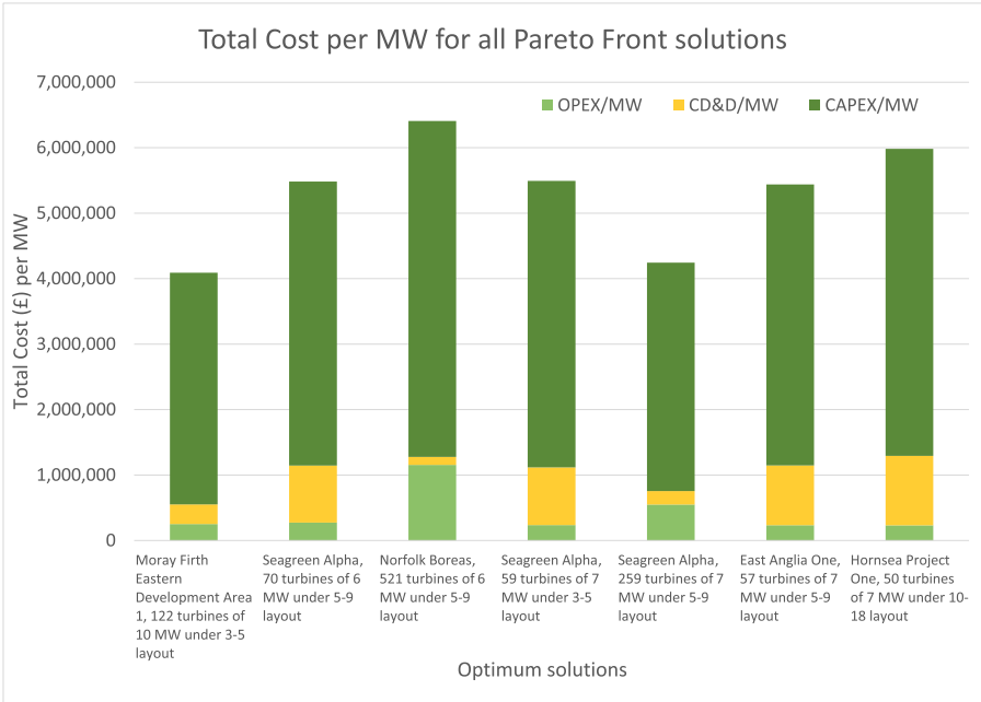
Fig. 9. Total Cost per MW for all Pareto Front solutions.
