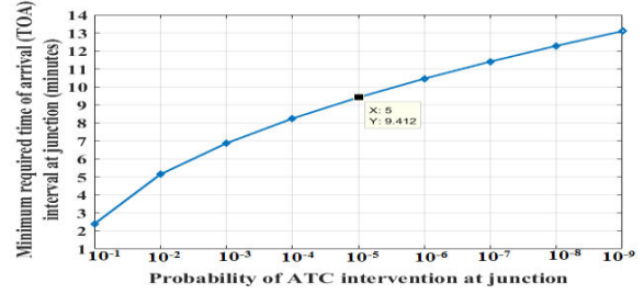
Fig. 2. TOA interval for different probabilities of ATC Intervention at Junction.
