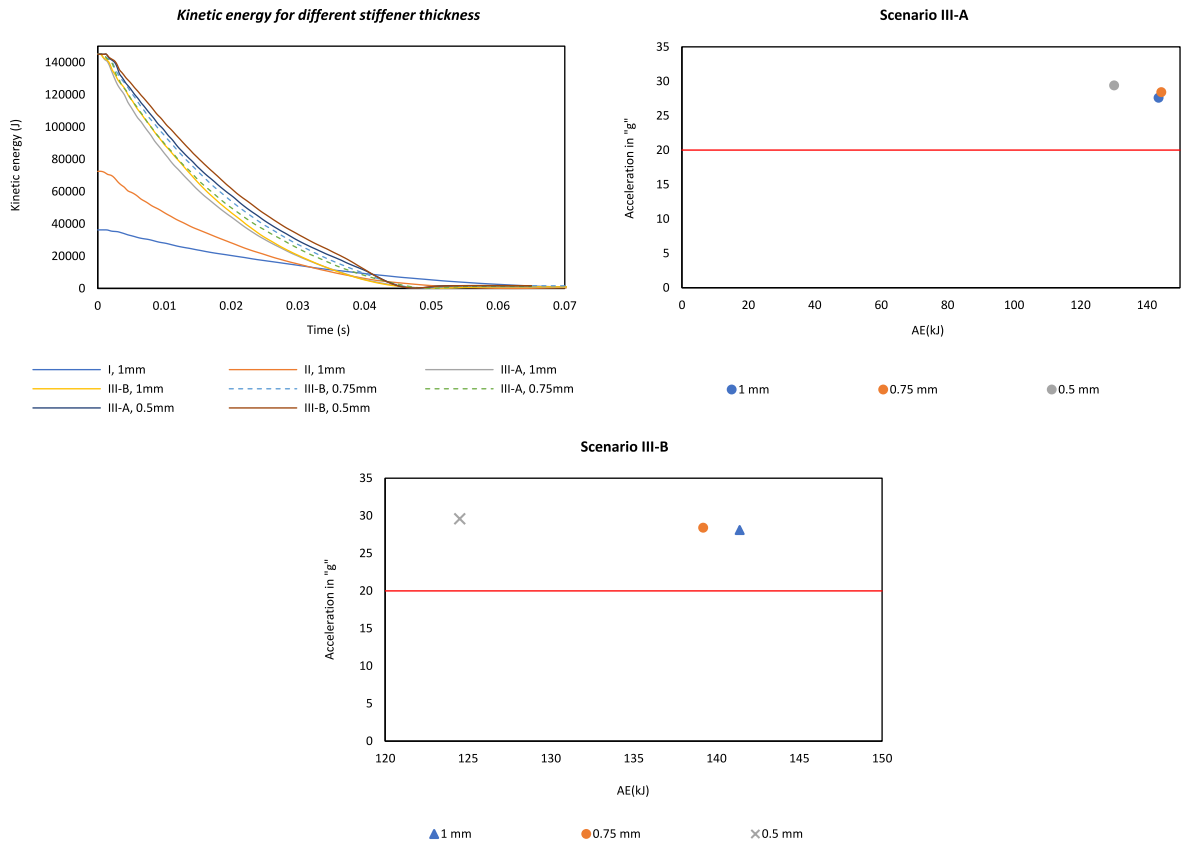
Fig. 26. KE evolution and comparison of AE and mean acceleration for various stiffener thicknesses and scenarios.
