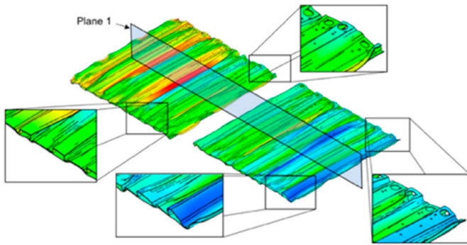
Fig. 22. Isometric view, U1 displacement on corrugated sheets and stiffeners, middle cell on the left, side cell on the right.
