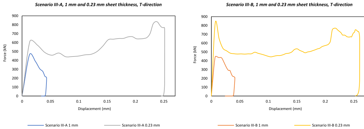
Fig. 16. Scenario III-A and III-B, FD diagrams, 1 mm and 0.23 mm sheet thickness, T-direction.
