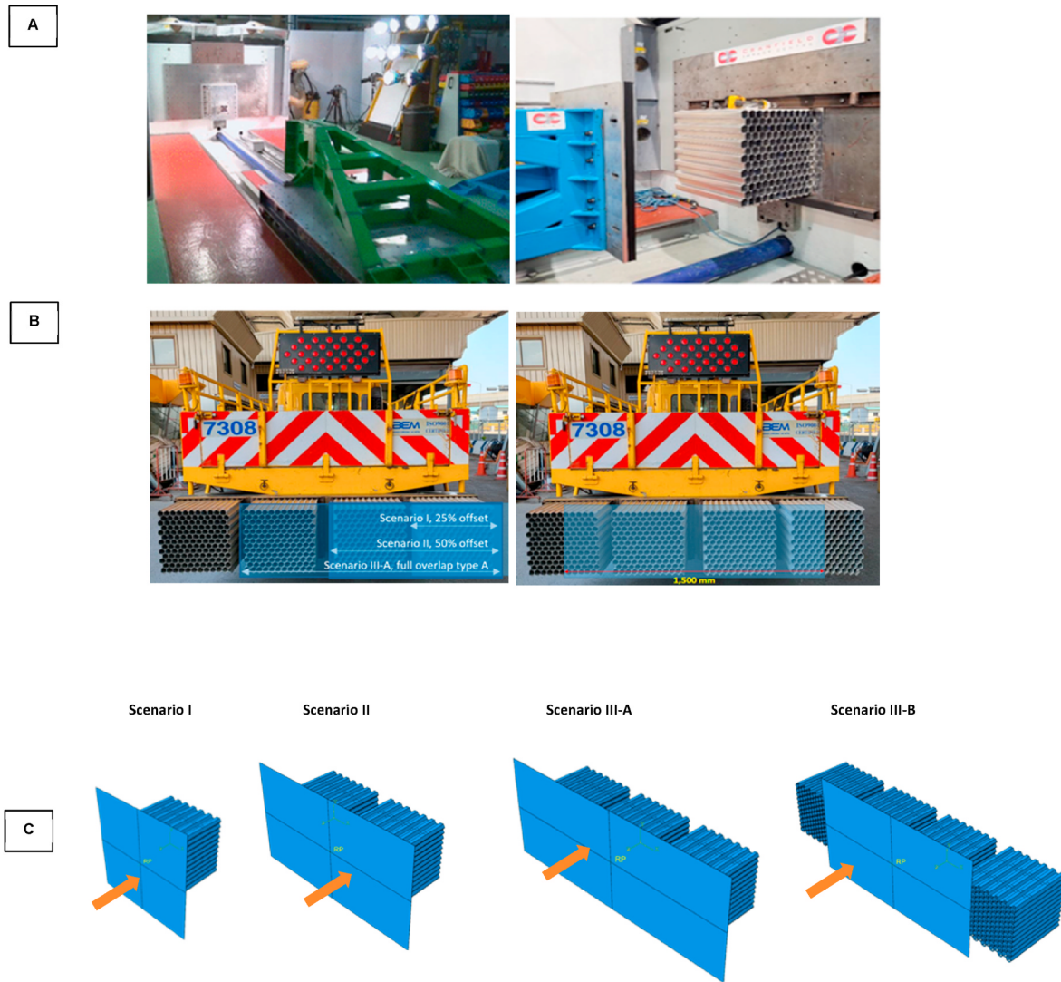
Fig. 3. A) Dynamic test set-up on an empty specimen at Cranfield Impact Centre (CIC), B) Test matrix of honeycomb absorbers, and C) Scenarios I, II and III-A, III-B.
