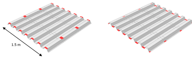
Fig. 4. Tie-constrained surfaces (in red) for modelling the welding joints. (For interpretation of the references to colour in this figure legend, the reader is referred to the Web version of this article.)
