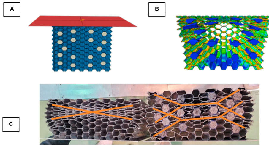
Fig. 8. A) Foam-filled honeycomb in L-direction impact, B) FEA and C) Experimental deformations.
