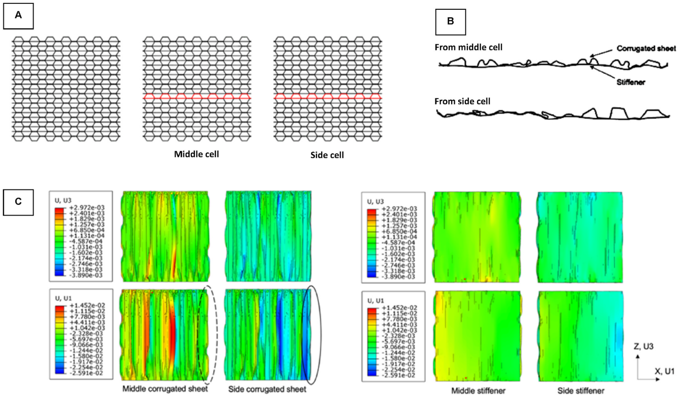
Fig. 21. A) Selected stiffeners and corrugated sheet in red, scenario III-A, profile view. B) Section view of the selected stiffeners and corrugated sheets in plane 1, and C) In-plane displacements U1 and U3 (in m) for the middle and side cells corrugated sheets and stiffeners. (For interpretation of the references to colour in this figure legend, the reader is referred to the Web version of this article.)
