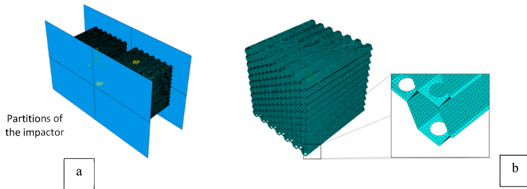
Fig. 5. a) Assembly for scenario II and b) meshed assembly systems.
