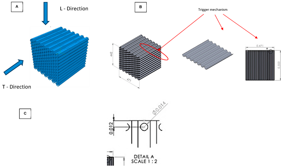
Fig. 1. A) Impact directions (T-direction is normal to the front face and L-direction is normal to the side of honeycomb absorber), B) CAD model and dimensions of the honeycomb, corrugated sheet, and C) trigger mechanism for the unreinforced honeycomb design.
