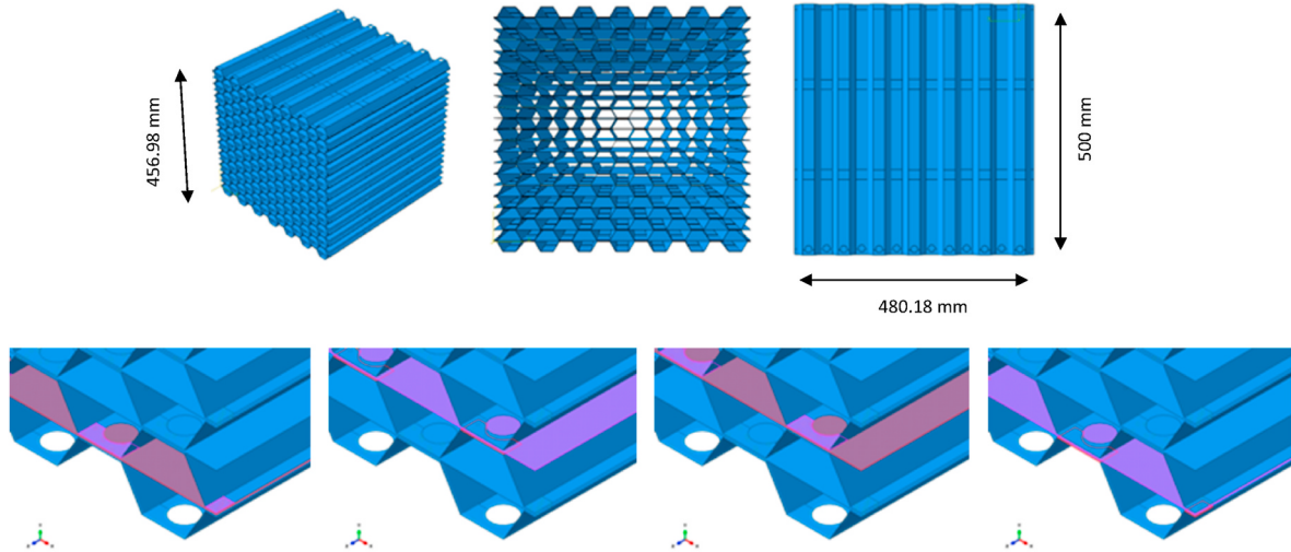
Fig. 12. Model of the reinforced honeycomb structure (top), successive master/slave in red (bottom). (For interpretation of the references to colour in this figure legend, the reader is referred to the Web version of this article.)
