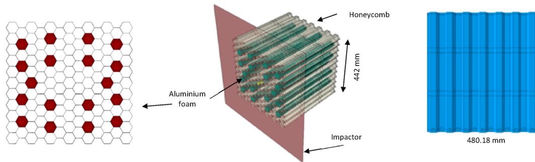
Fig. 6. Foam-filled honeycomb and corrugated sheets, also for validation purposes.
