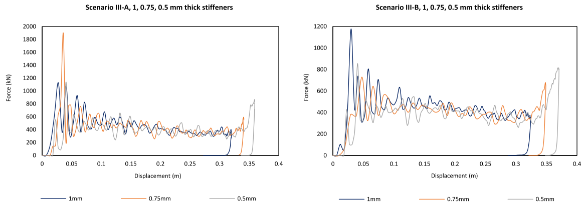
Fig. 25. Force displacement diagrams with various scenarios and thicknesses for stiffeners, L-direction impact.
