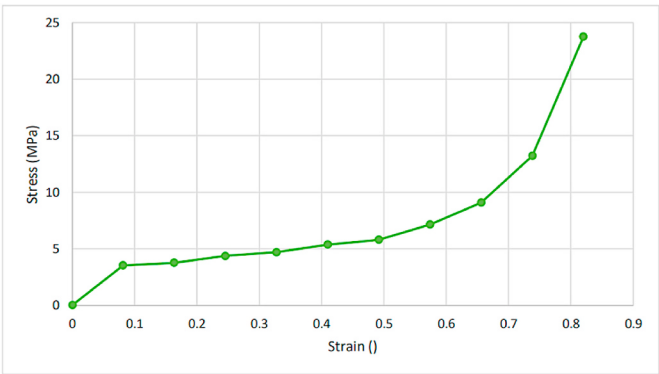
Fig. 2. Aluminium model stress-strain curve.
