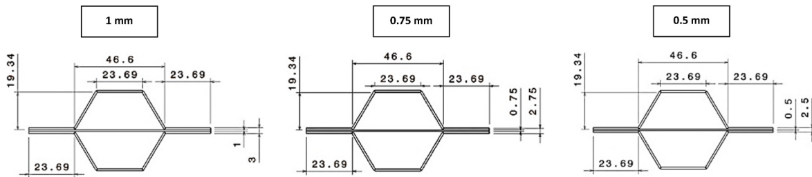
Fig. 13. Hexagonal cell geometry with 1 mm sheet thickness and 1 mm, 0.75 mm, 0.5 mm stiffener thickness.
