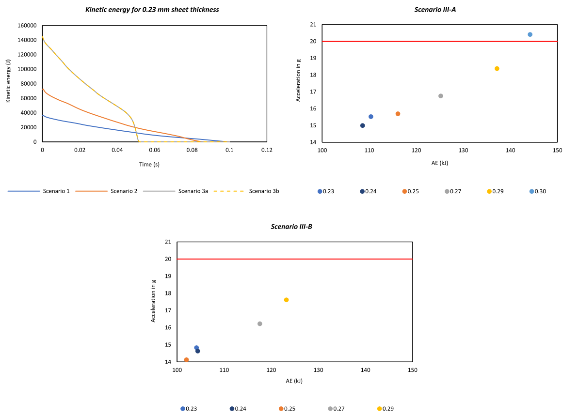
Fig. 20. KE evolution, comparison of AE and MA for various thicknesses (mm) and scenarios.
