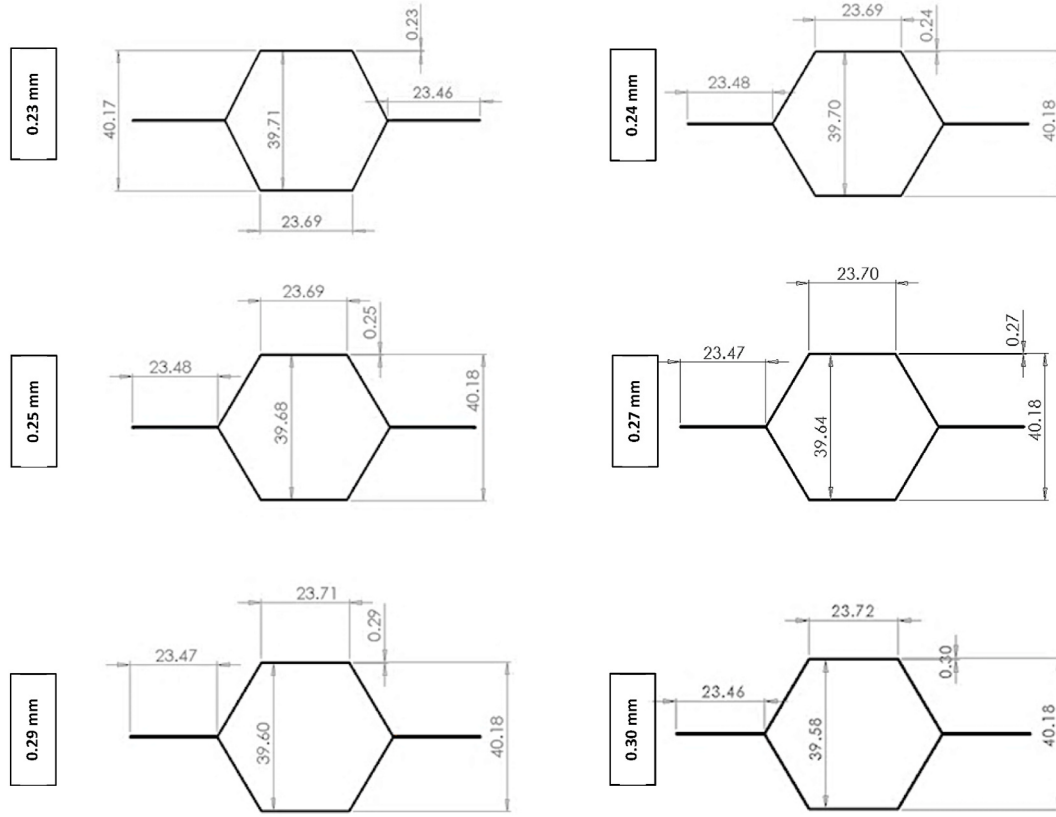
Fig. 11. The geometry of the hexagonal cell with 0.23 mm, 0.24 mm, 0.25 mm, 0.27 mm, 0.29 mm, and 0.30 mm corrugated sheet thickness.
