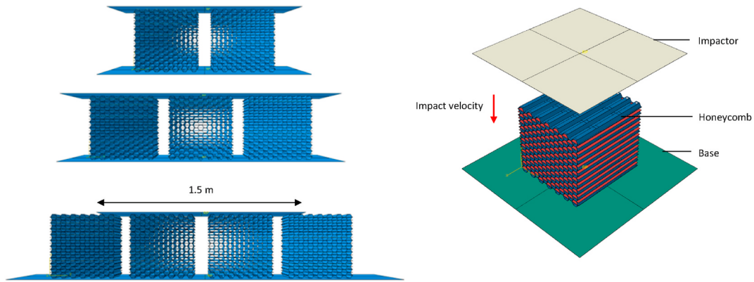
Fig. 14. FEM model for each scenario with stiffener-reinforced designs.
