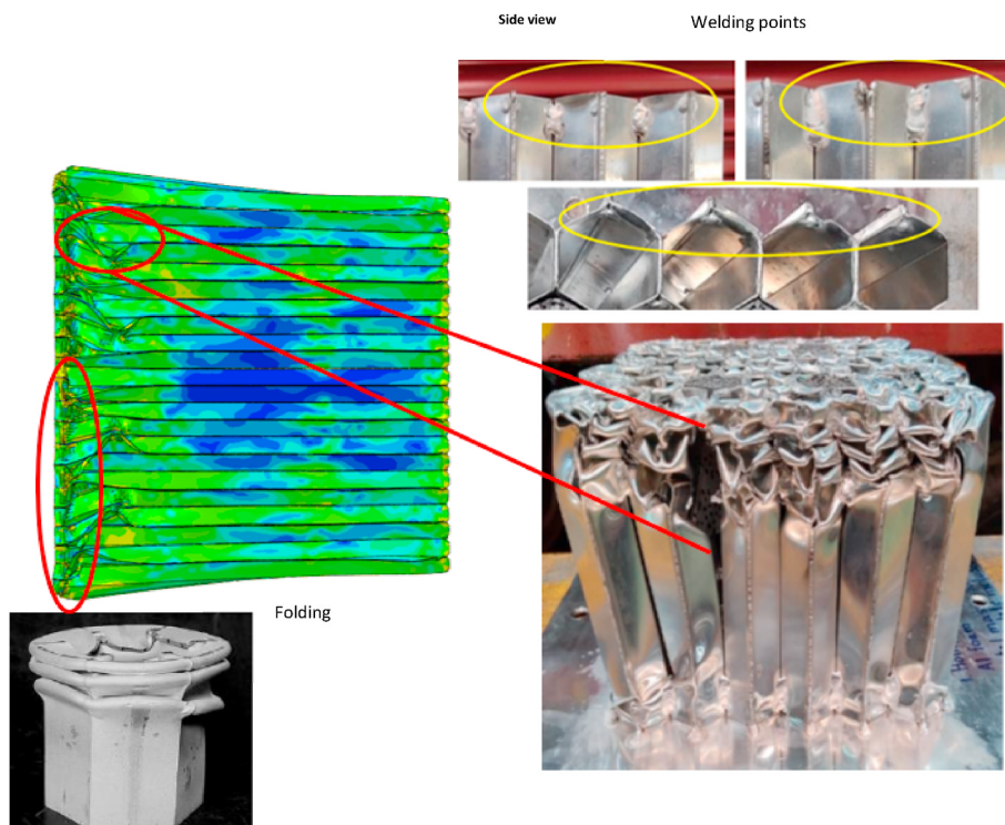
Fig. 10. Comparison of simulated (calibrated model) and experimental deformations, T-direction impact.
