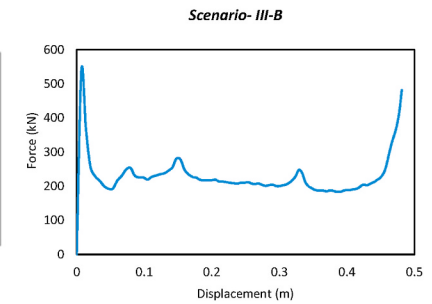
Fig. 18. Von-Mises stress distributions in intermediate crushing state (left) and FD diagrams (right), all scenarios in T-direction impact, 0.23 mm thick sheets.
