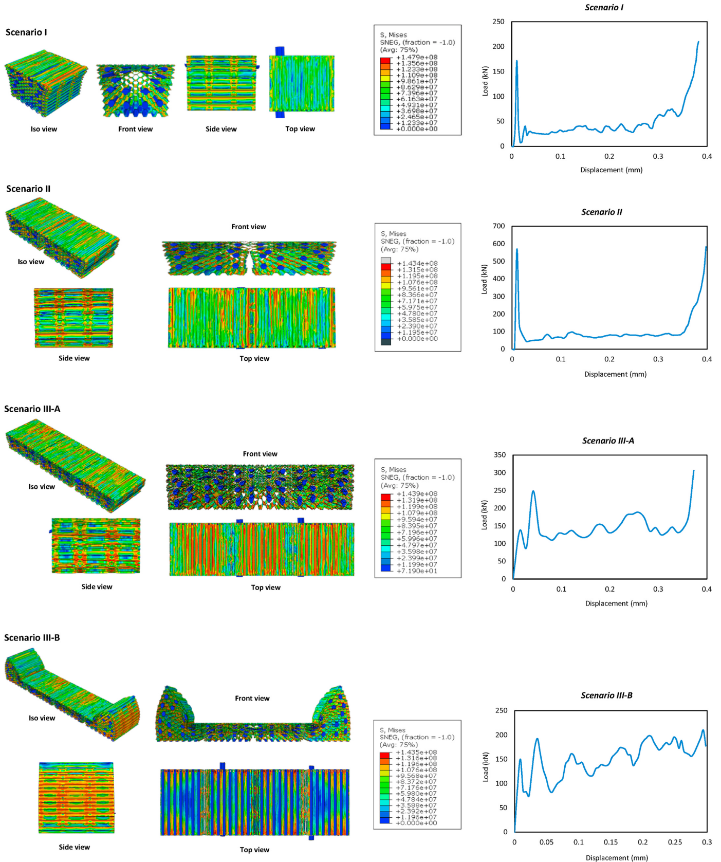
Fig. 17. Von-Mises stress distributions in the final crushing stage (left) and FD diagrams (right), all scenarios in L-direction impact, 1 mm thick sheets with aluminium foam fillers.
