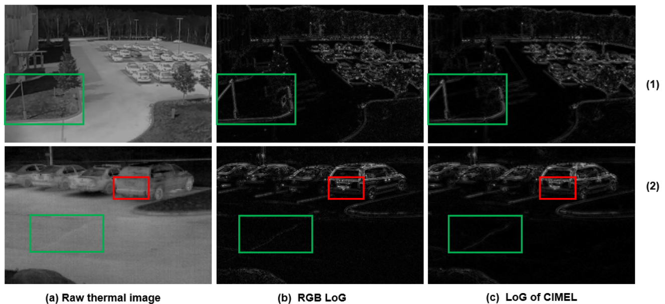
Figure 7. Two types of edges from the LoG algorithm: Edges weak in the IR spectrum but strong in the corresponding visual image (red rectangle); Edges which are strong in both IR and visual images (green rectangle).
