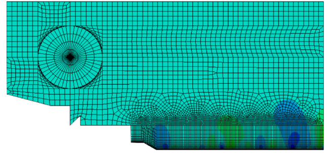
Fig. 11. RS distribution at the end of the iteration process on HAZ 2.
