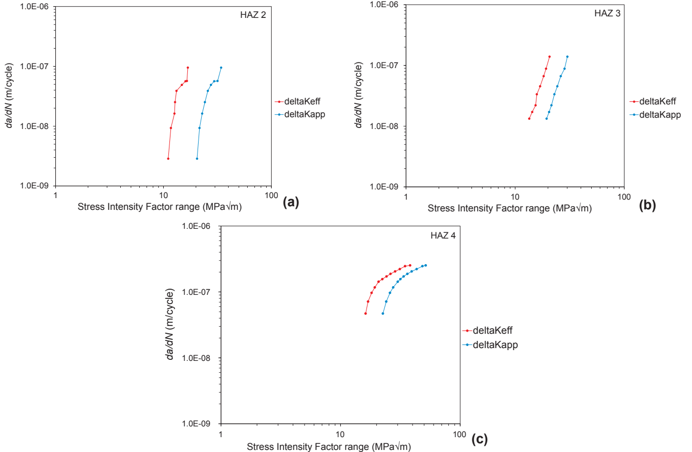
Fig. 15. Numerical and experimental FCG behaviour of (a) HAZ 2, (b) HAZ 3 and (c) HAZ 4.
