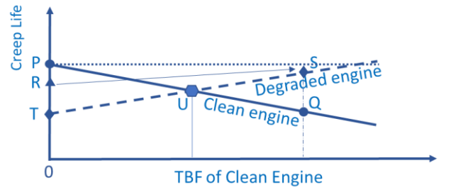
(c) ECF vs TBF
