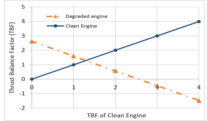
Figure 16: TBF of both engines at cruise condition
