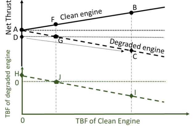
(a) Net Thrust vs TBF
