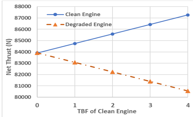
Figure 13: Net thrust vs TBF at cruise condition
