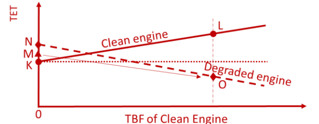
(b) TET vs TBF
