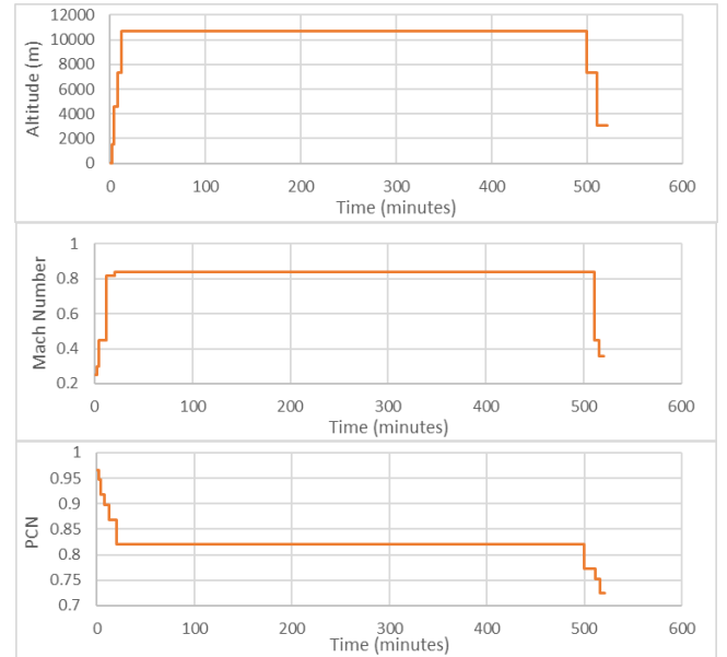
Figure 9. Flight mission profile
