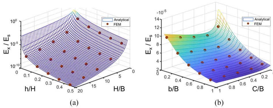
Figure 3. Variation of effective elasticity modulus in x -direction for a Fish Cell metamaterial with t = 0.01B and W = B with respect to (a) aspect ratio of the cell and vertical component of inclined rib's length for C = 0.1B and b = 0.5B , (b) connector's length and horizontal component of rib's length for H = B and h = 0.25H .
