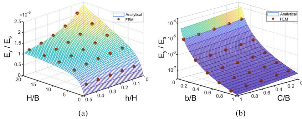
Figure 5. Variation of effective elasticity modulus in y -direction for a Fish Cell metamaterial with t = 0.01B and W = B with respect to (a) aspect ratio of the cell and vertical component of inclined rib's length for C = 0.1B and b = 0.5B and (b) connector's length and horizontal component of rib's length for H = B and h = 0.25H .
